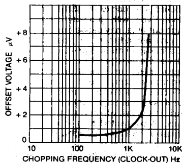
INPUT OFFSET VOLTAGE vs. CHOPPING FREQUENCY
