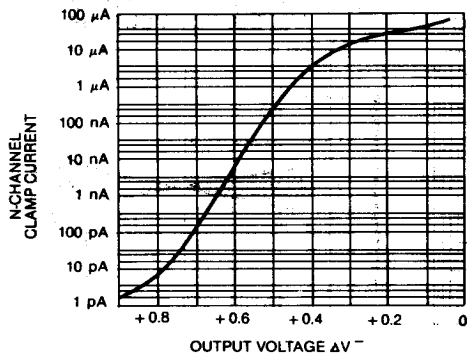
N-CHANNEL CLAMP CURRENT vs. OUTPUT VOLTAGE
