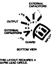
SUGGESTED BOARD LAYOUT AM-7650-2
