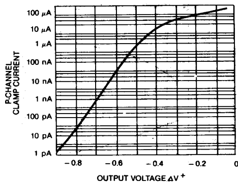
P-CHANNEL CLAMP CURRENT vs. OUTPUT VOLTAGE
