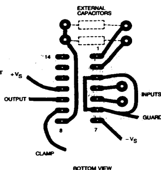
SUGGESTED BOARD LAYOUT AM-7650-1
