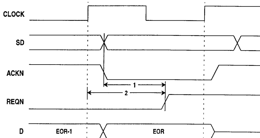
Figure 18: Request Deasserts at EOR, Strobe Condition of DSC=0-3, 6-15; ERC=0
