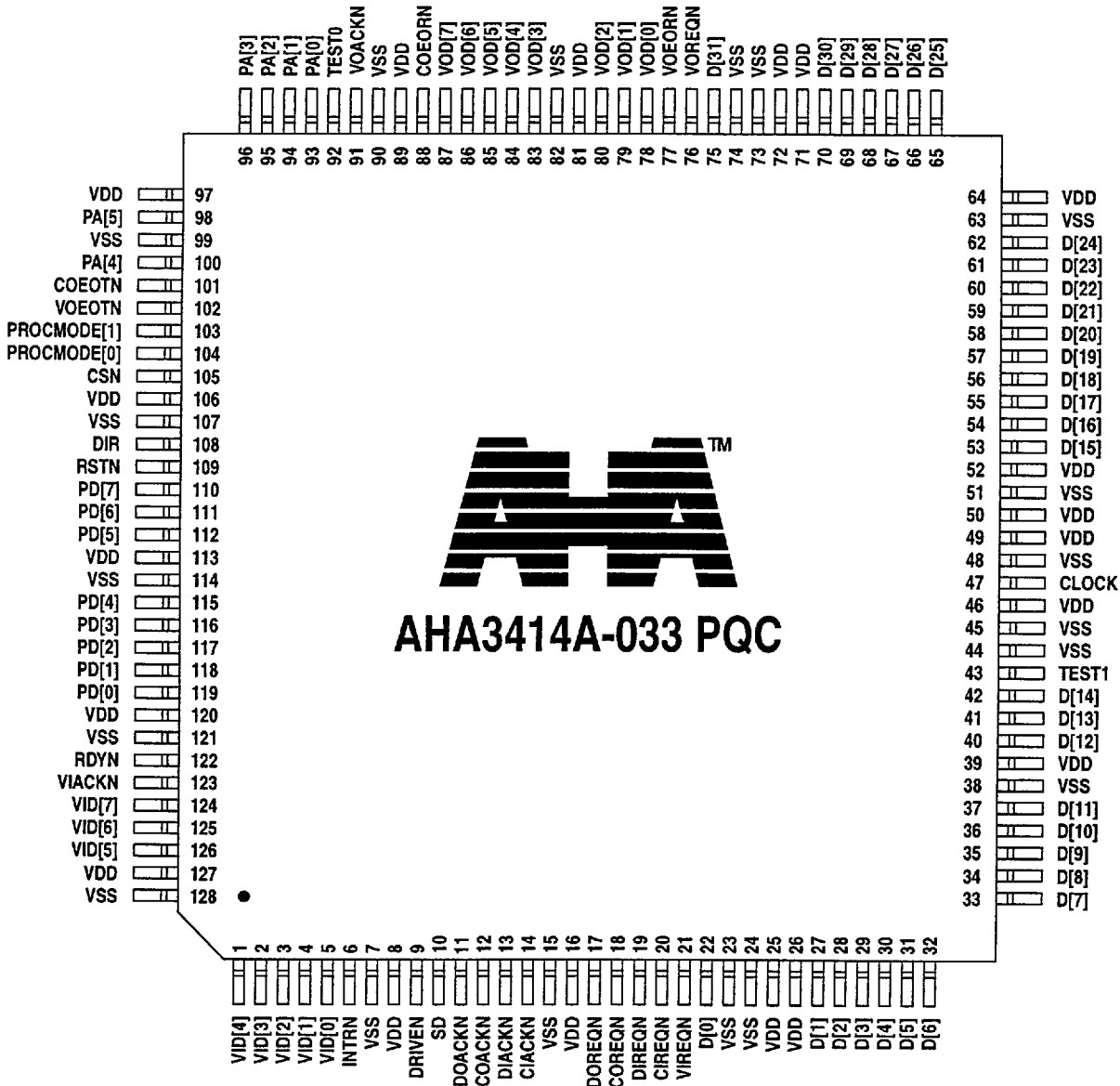
Figure 16: Pinout
