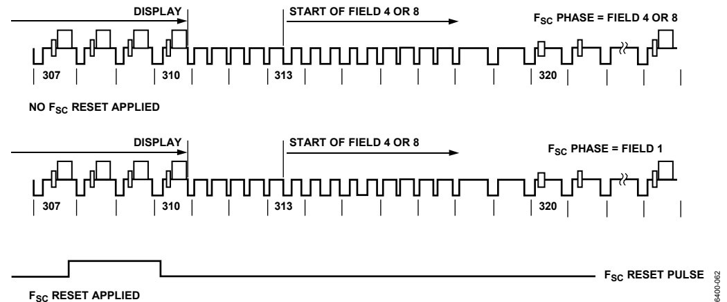
Figure 61. SD Subcarrier Phase Reset Timing Diagram (Subaddress 0x84, Bits[2:1] = 01)
