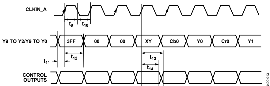
Figure 13. ED Only (at 54 MHz), 8-/10-Bit, 4:2:2 YCrCb (EAV/SAV) Pixel Input Mode (Input Mode 111)
