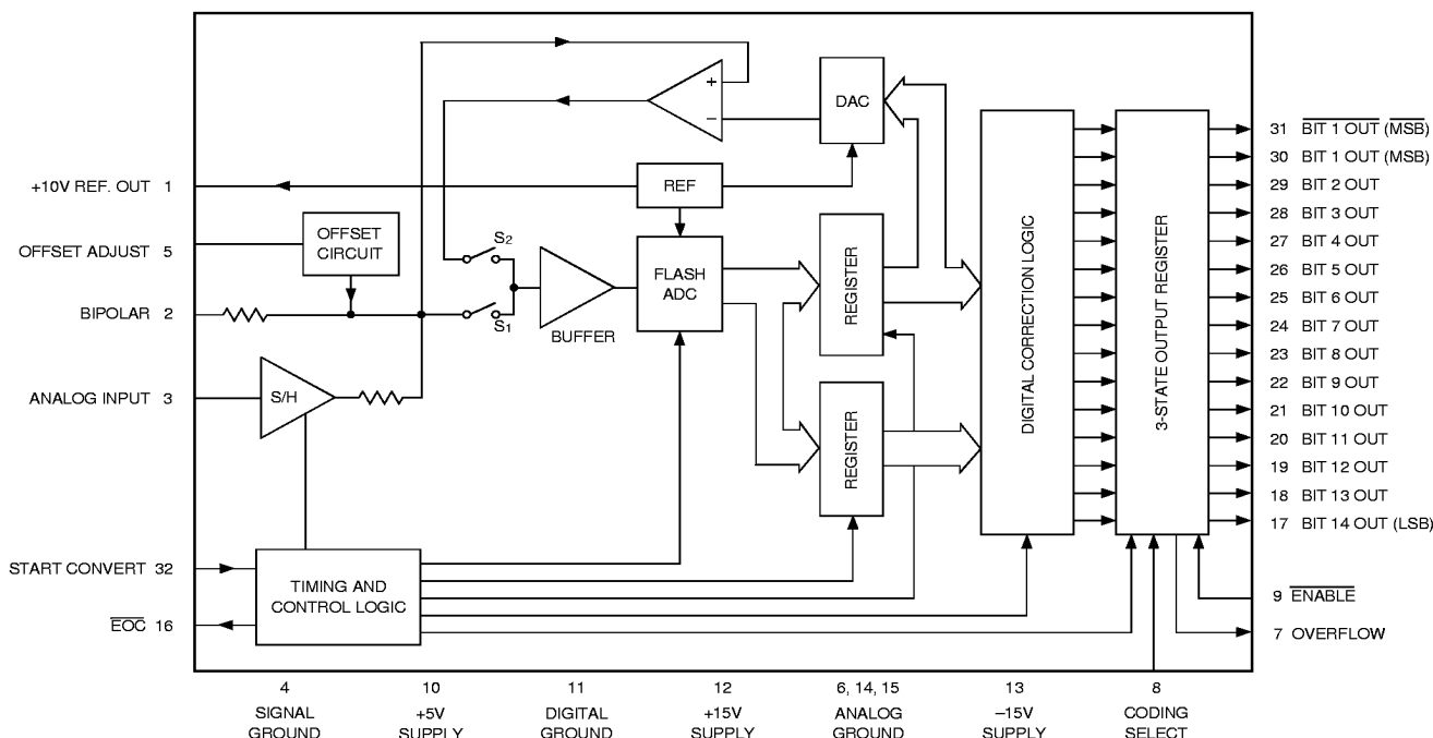
Figure 1. ADS-941 Functional Block Diagram
