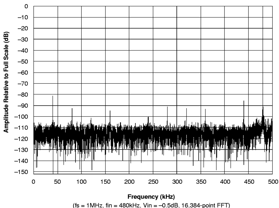
Figure 4. FFT Analysis of ADS-941
