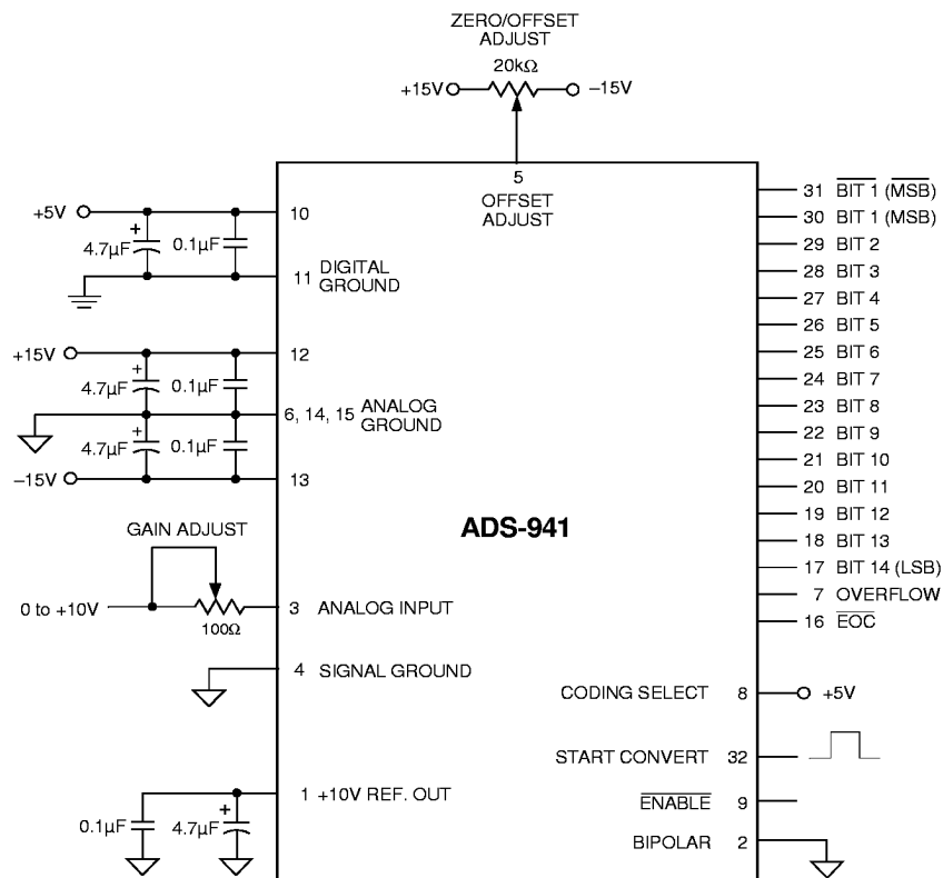
Figure 3. ADS-941 Connection Diagram
