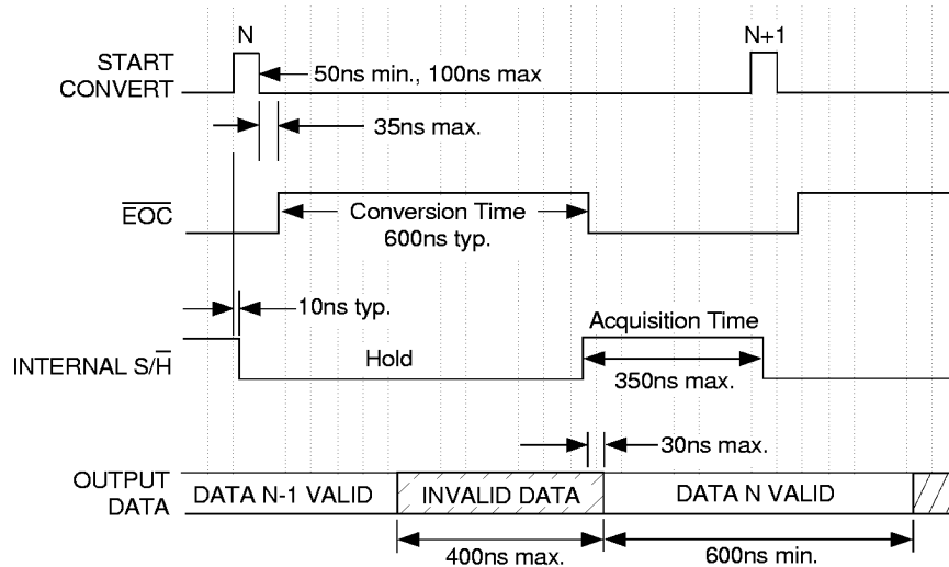
Figure 2. ADS-941 Timing Diagram
