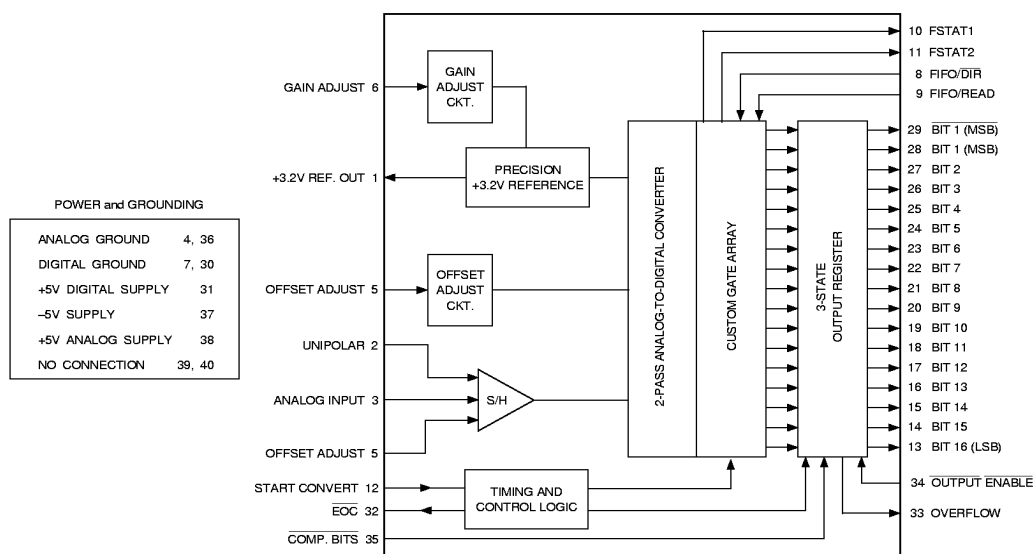
Figure 1. ADS-931 Functional Block Diagram
