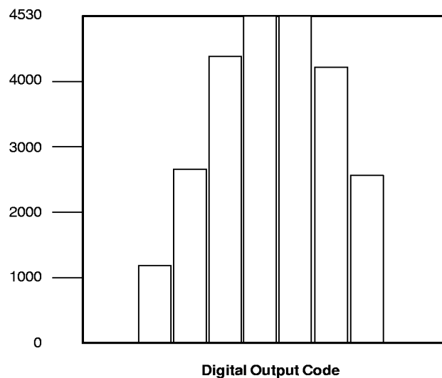
Figure 6. ADS-931 Grounded Input Histogram
