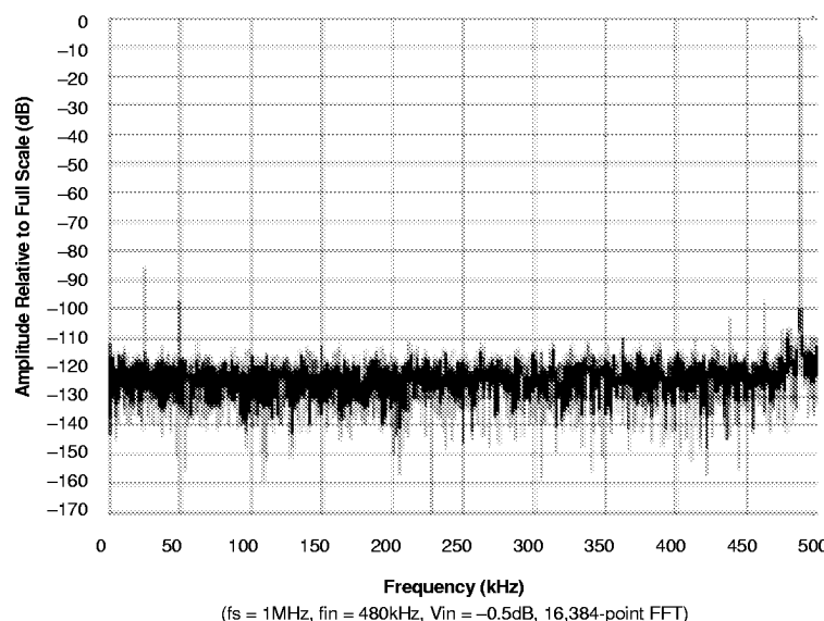
Figure 4. FFT Analysis of ADS-931
