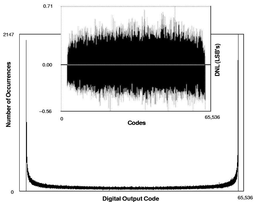
Figure 5. ADS-931 Histogram and Differential Nonlinearity
