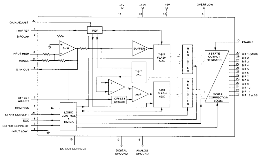
Figure 1. ADS-132 Simplified Block Diagram
