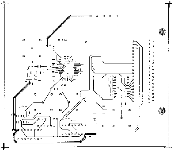
Figure 41. Conductors—Top View
