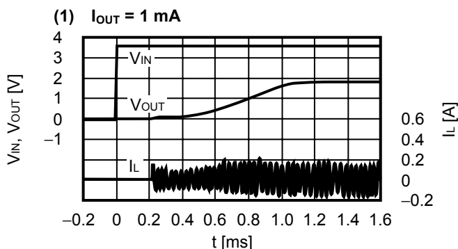
3.1 Powering ON ( V_{OUT} = 1.8 \text{ V} , V_{IN} = 0 \text{ V} \rightarrow 3.6 \text{ V} , T_a = 25^\circ\text{C} )
