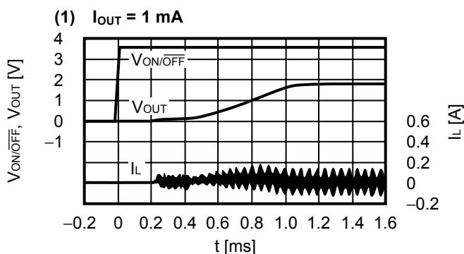
3.2 Shutdown pin response ( V_{OUT} = 1.8 \text{ V} , V_{IN} = 3.6 \text{ V} , V_{ON/OFF} = 0 \text{ V} \rightarrow 3.6 \text{ V} , T_a = 25^\circ\text{C} )
