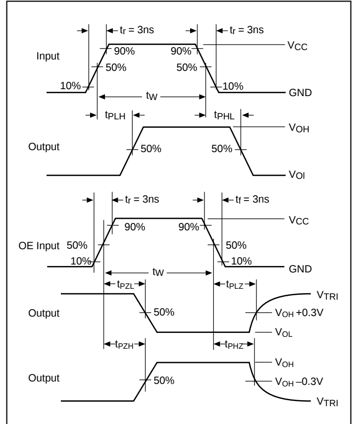
Figure 3. AC Waveforms
