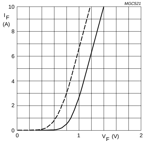
BYV28-300 and 400 Dotted line: T_j = 175\text{ °C} . Solid line: T_j = 25\text{ °C} .
