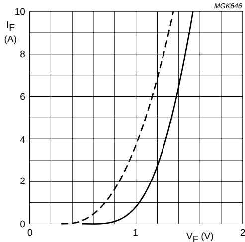
BYV28-500 and 600 Dotted line: T_j = 175\text{ °C} . Solid line: T_j = 25\text{ °C} .
