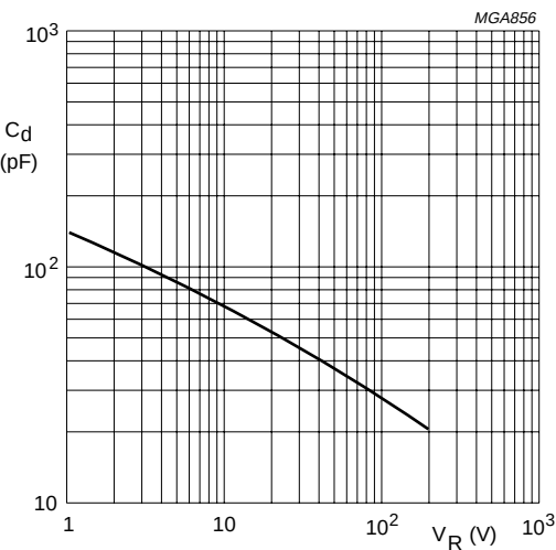
BYV28-50 to 200 f = 1\text{ MHz} ; T_j = 25\text{ °C} .
