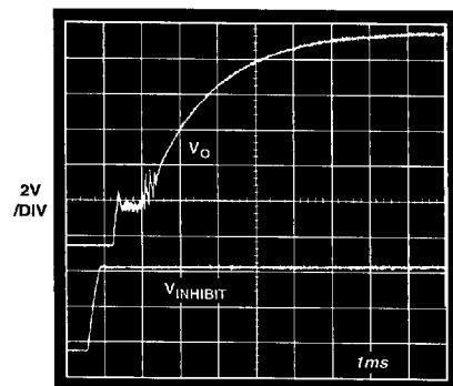
Figure 6. Output Voltage Transient During Turn-On with Minimum Load Displaying Soft Start When Supply Is Enabled
