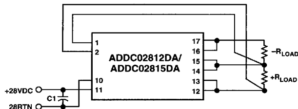
Figure 28. Typical Power Connections and External Parts for Converter
