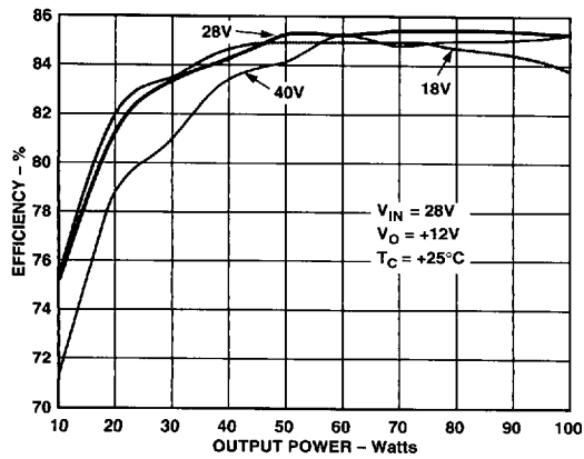
Figure 1. Efficiency vs. Line and Load at +25°C (ADDC02812DA)
