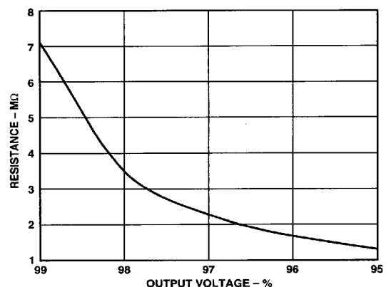
Figure 18. External Resistor Value for Reducing Output Voltage
