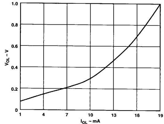
Figure 21. Sink Capability of Status Output
