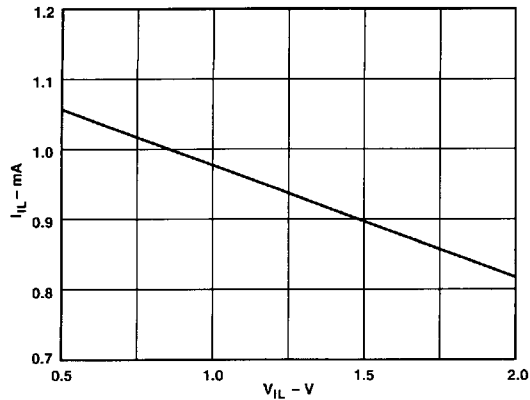
Figure 23. Input Characteristics of Pin 6 When Pulled Low
