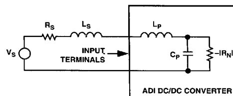
Figure 25. Model of Power Source and POL Converter Connection
