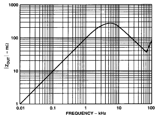
Figure 11. Incremental Output Impedance (Magnitude)
