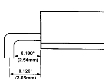
Figure 27. Minimum Bend Radius of 40 Mil (1.02 mm) Pins
