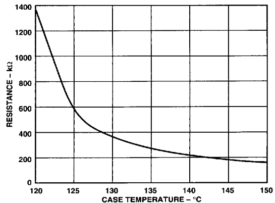
Figure 24. External Resistor Value for Raising Temperature Shutdown Point
