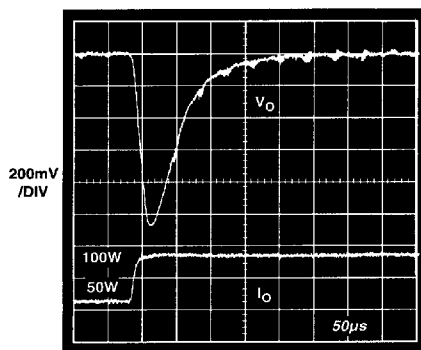
Figure 7. Output Voltage Transient Response to a 50% to a 100% Step Change in Load with Zero Load Capacitance (ADDC02812DA)
