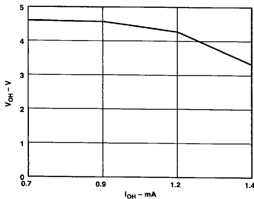
Figure 20. Source Capability of Status Output
