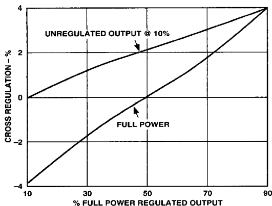
Figure 9. Cross Regulation Envelope
