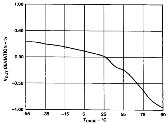
Figure 5. Normalized Output Voltage vs. Case Temperature (°C)
