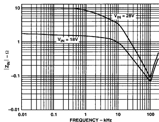
Figure 12. Incremental Input Impedance (Magnitude)
