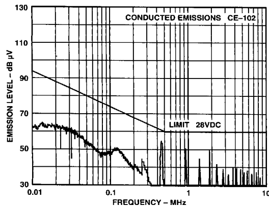
Figure 14. Conducted Emissions, MIL-STD-461D, CE102, +28 V Hot Line 100 W Load
