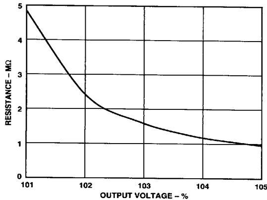
Figure 19. External Resistor Value for Increasing Output Voltage
