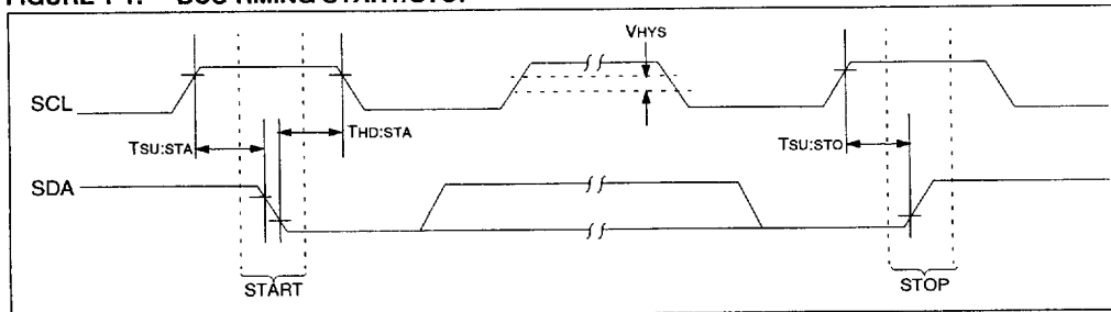
FIGURE 1-1: BUS TIMING START/STOP
