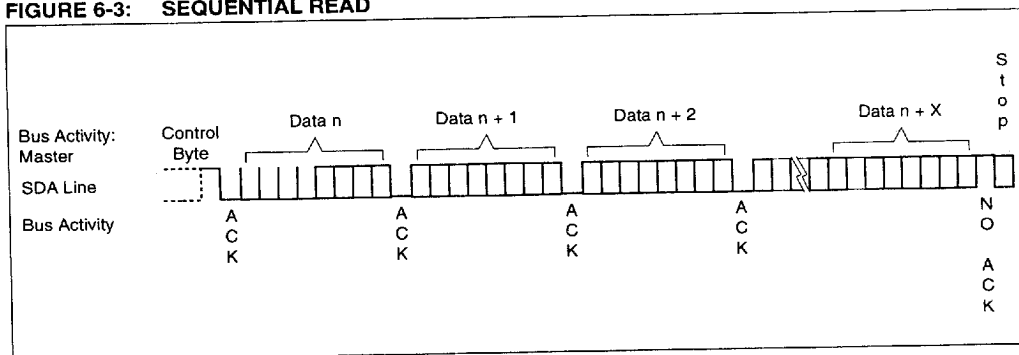
FIGURE 6-3: SEQUENTIAL READ
