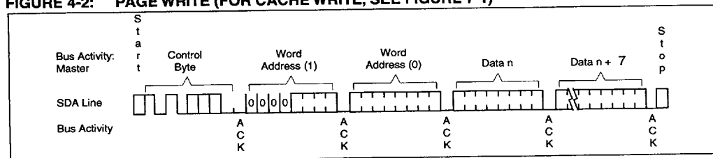
FIGURE 4-2: PAGE WRITE (FOR CACHE WRITE, SEE FIGURE 7-1)
