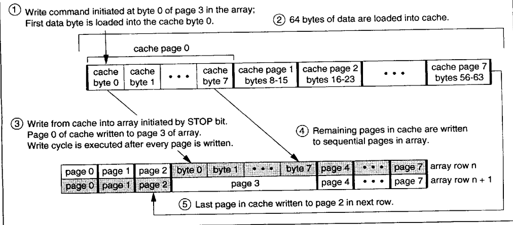
FIGURE 7-2: CACHE WRITE TO THE ARRAY STARTING AT A NON-PAGE BOUNDARY
