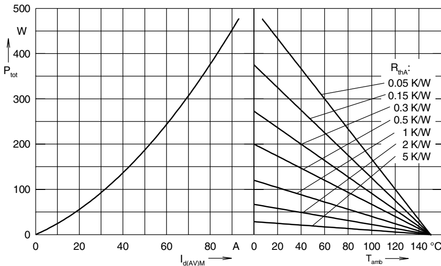
Fig. 4 Power dissipation versus direct output current and ambient temperature, sin 1/8
