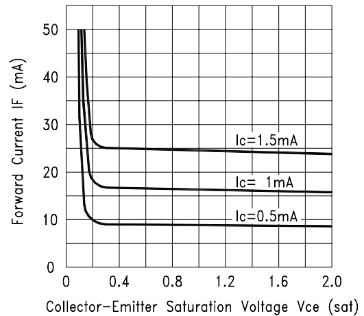
Fig.4 FORWARD CURRENT VS. Collector-Emitter Saturation Voltage
