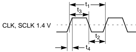
Figure 5.5 External Clock
