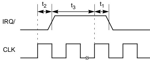
Figure 5.7 Interrupt Output
