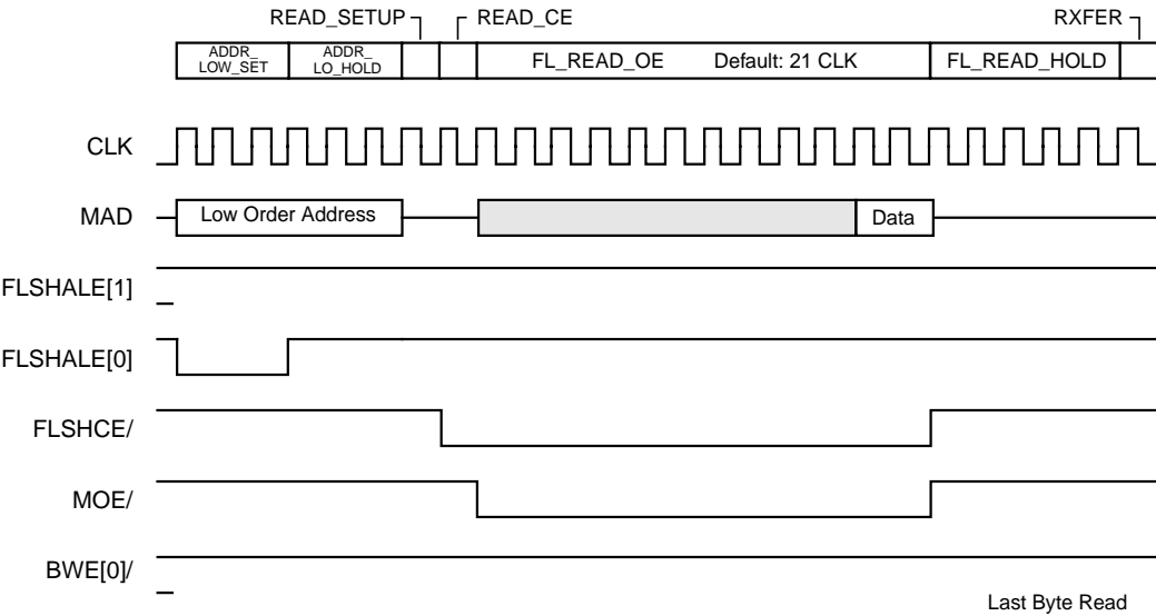
Figure 5.9 Flash ROM Read Timing
