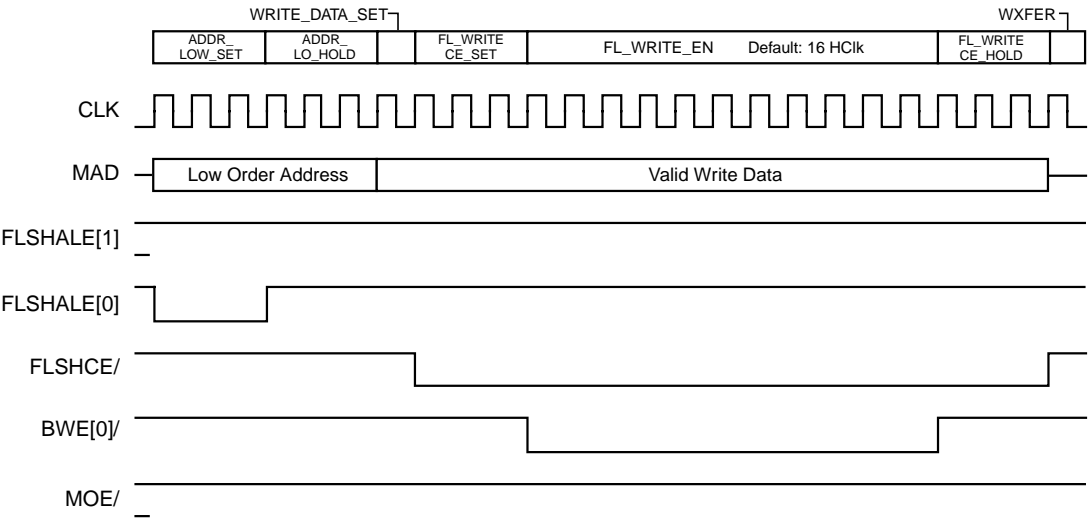
Figure 5.10 Flash ROM Write Timing
