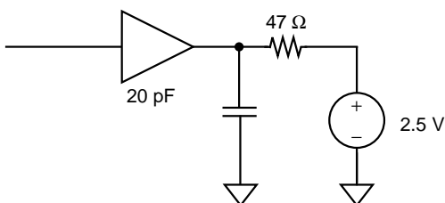
Figure 5.3 Rise and Fall Time Test Condition
