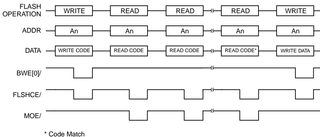
Figure 5.11 Flash ROM Polling
