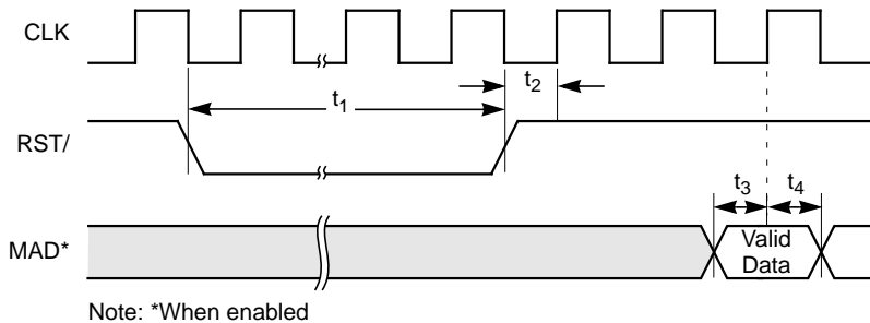
Figure 5.6 Reset Input
