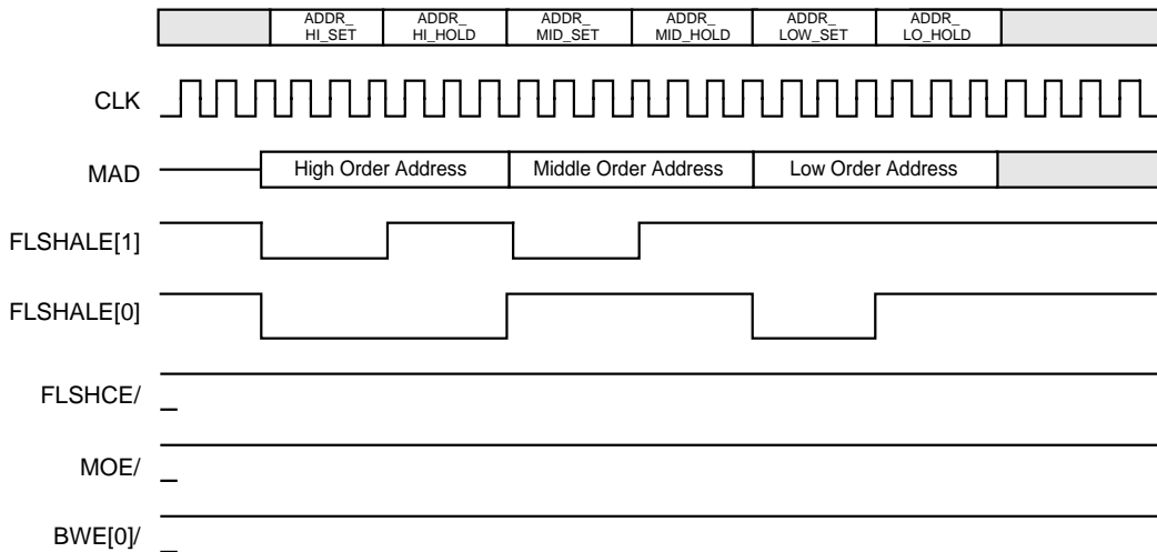
Figure 5.8 Flash ROM Address Timing
