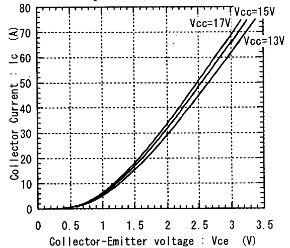
Collector current vs. Collector-Emitter voltage T_j=125^\circ\text{C} (Terminal)
