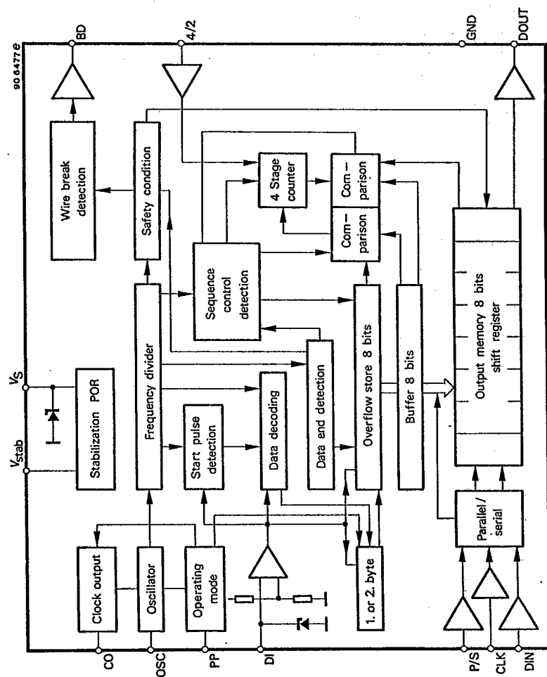
Fig. 2 Block diagram U 6056 B
