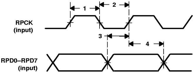
Figure 8. Receive High-Speed Interface
