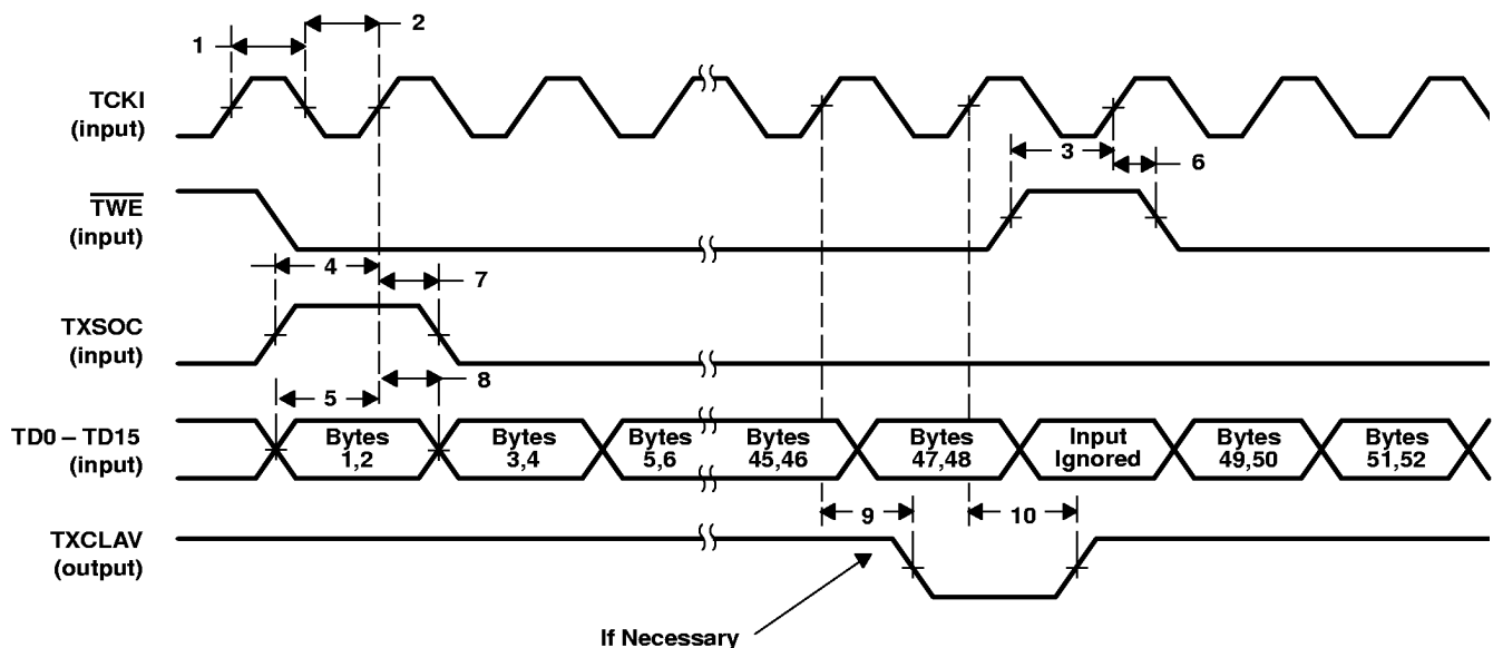
Figure 5. Transmit-Cell Interface
