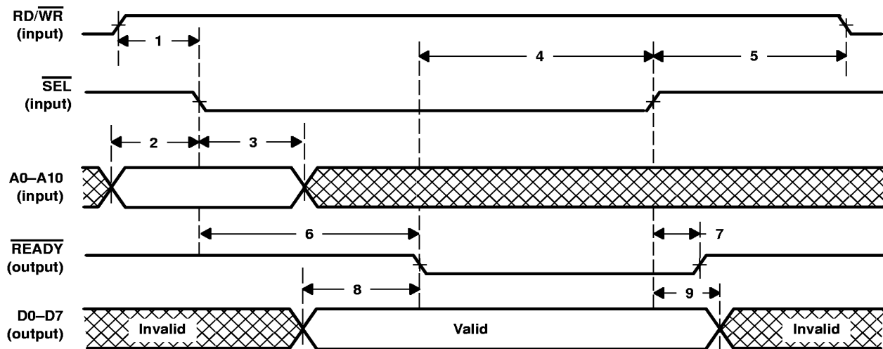
Figure 11. Controller-Interface Read Cycle
