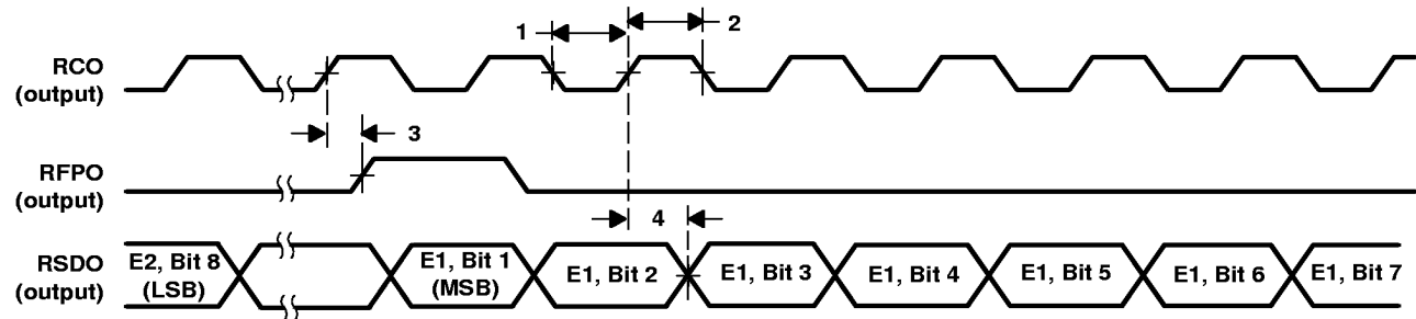
Figure 9. Receive Data-Communications Interface
