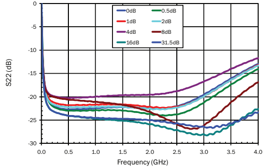
RF2 RL versus Frequency, Major States
