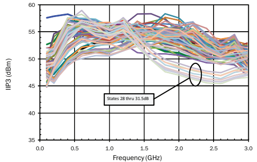
Input IP3 versus Frequency, All States, 25C
