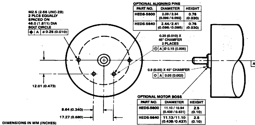
Figure 4. Mounting with External Ears.
