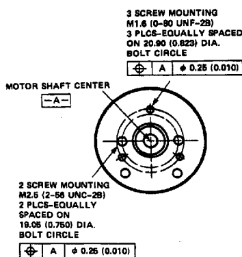
Figure 2. Mounting Holes.
