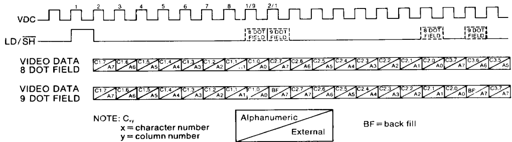
FIGURE 4 TYPICAL VIDEO OUTPUT
