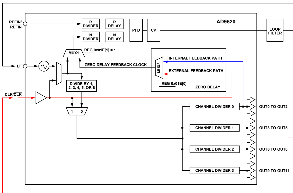
Figure 48. Zero Delay Function
