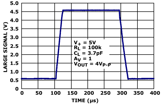
FIGURE 30. LARGE SIGNAL STEP RESPONSE (4V)
