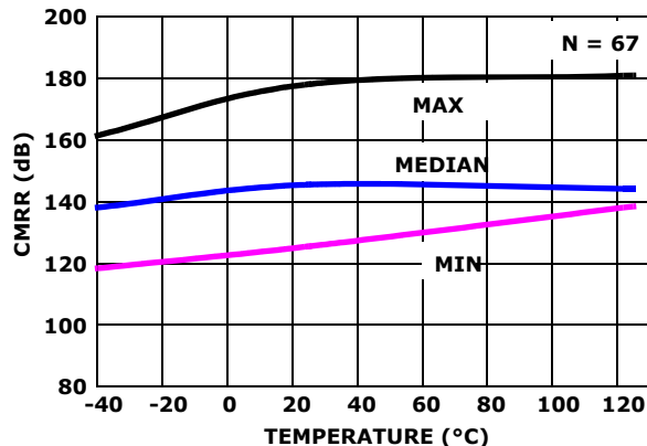
FIGURE 28. CMRR vs TEMPERATURE, V CM = -2.5V TO +2.5V, V+ = ±2.5V
