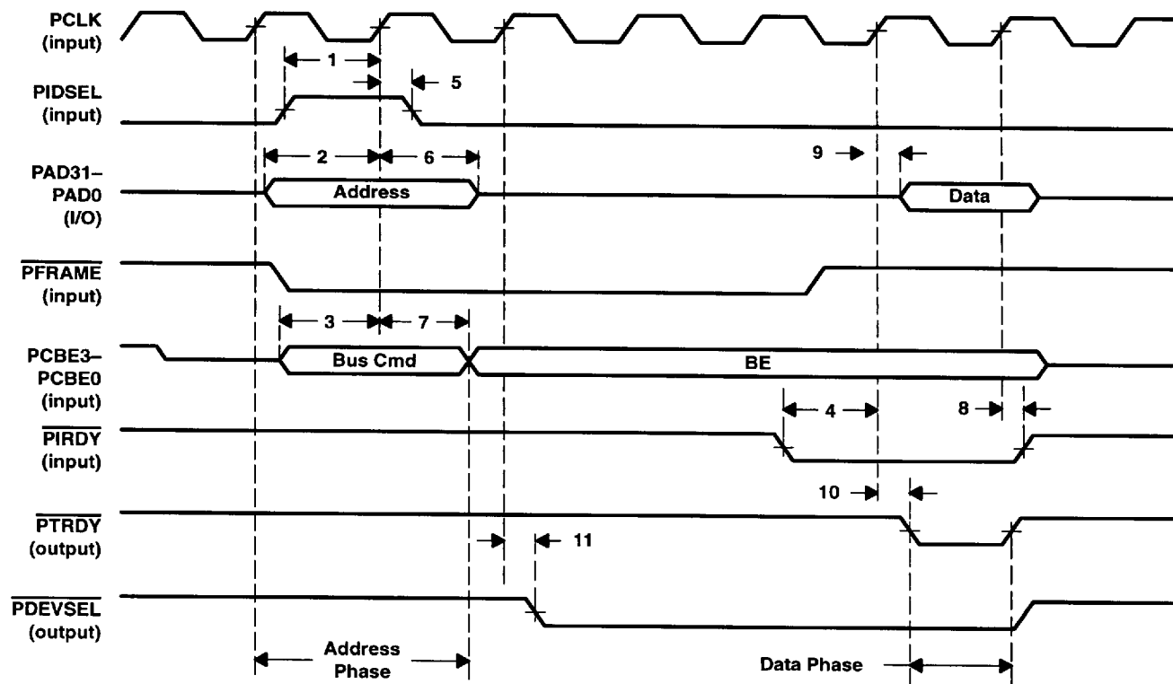
Figure 7. TNETA1570 Read Operation (PCI SAR as Slave)
