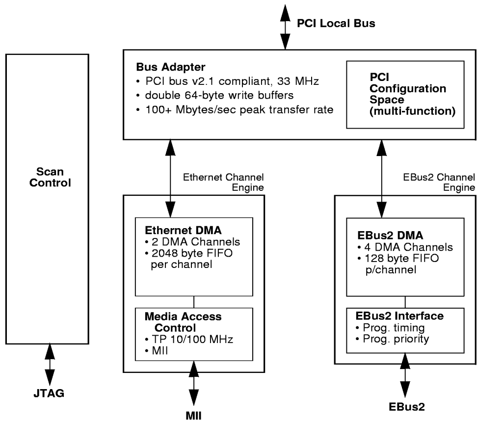
Figure 1. PCIO Block Diagram
