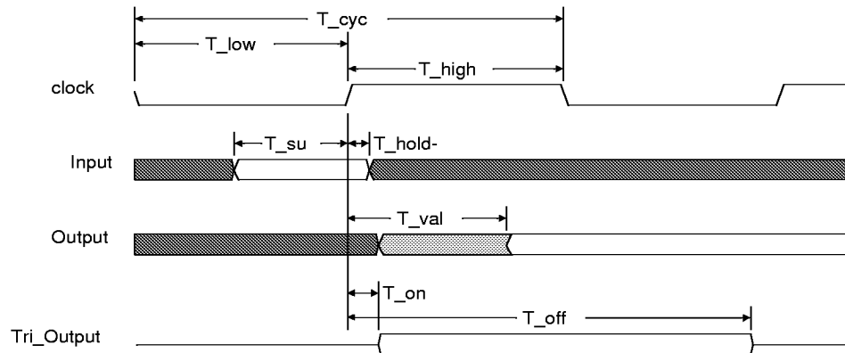
Figure 3. General Timing Waveforms
