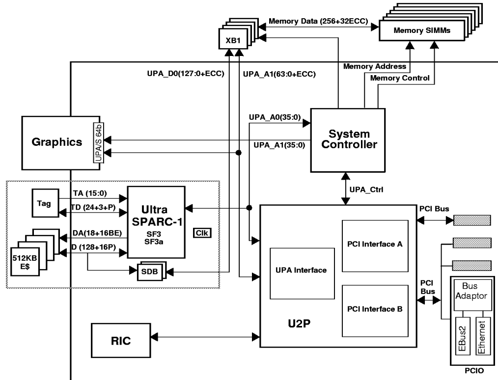
Figure 2. Typical System Application
