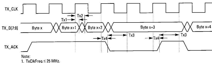
Figure 9. TX_D[7:0] and TX_ACK
