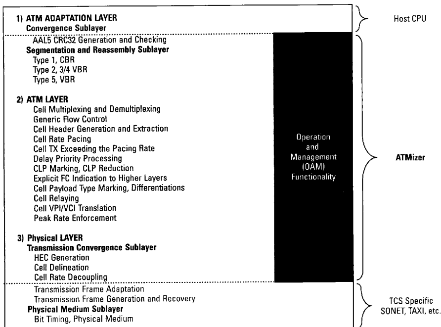
Figure 2. ATMizer-Supported ATM Layers
