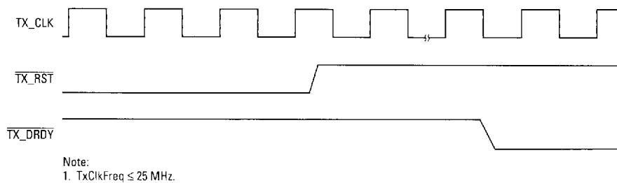
Figure 11. TX_RST
