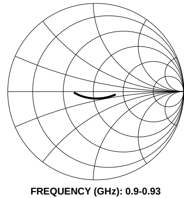
Figure 15. Input Impedance.
