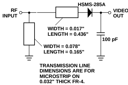
Figure 17. 2.45 GHz Matching Network for the HSMS-285A Series.
