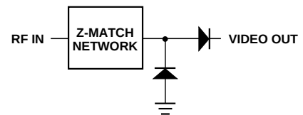
Figure 28. Voltage Doubler Circuit.
