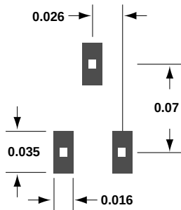
Figure 32. PCB Pad Layout (dimensions in inches).
