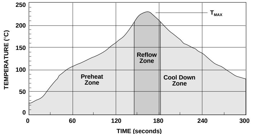
Figure 33. Surface Mount Assembly Profile.
