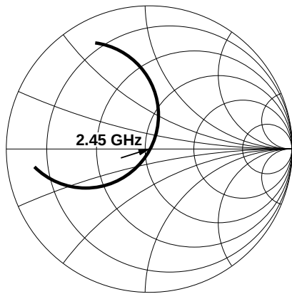
Figure 23. Input Impedance. Modified 2.45 GHz Circuit.
