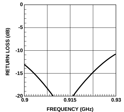
Figure 16. Input Return Loss.
