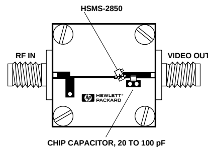
Figure 20. Test Detector.
