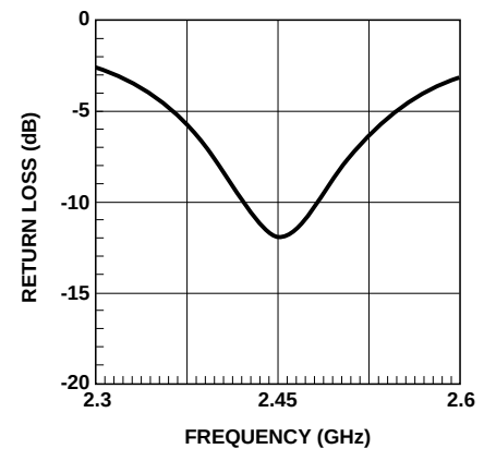
Figure 22. Input Return Loss.
