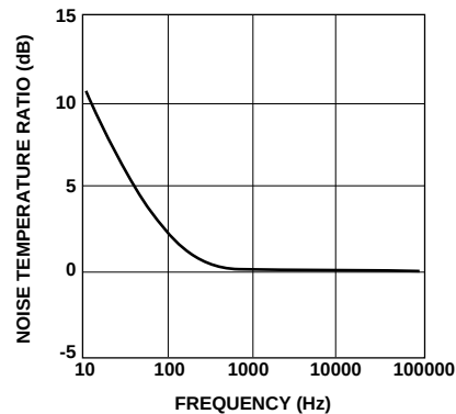
Figure 29. Typical Noise Temperature Ratio.
