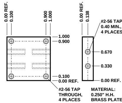
Figure 19. Mounting Plate.
