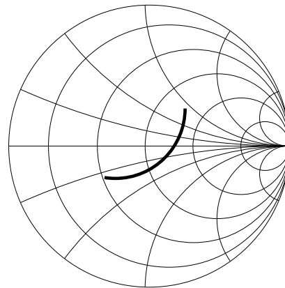
Figure 26. Input Impedance.
