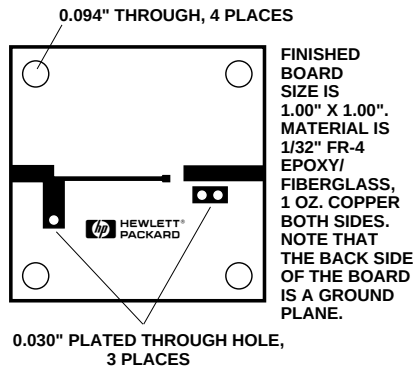
Figure 18. Physical Realization.
