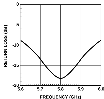
Figure 27. Input Return Loss.
