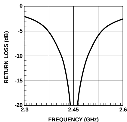
Figure 24. Input Return Loss. Modified 2.45 GHz Circuit.
