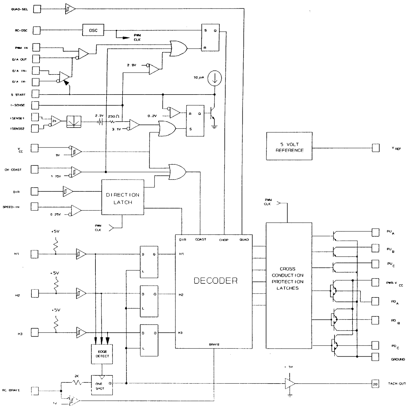
FIGURE 2. Block diagram.
