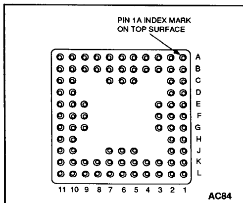
Fig.1 Pin connections - bottom view (AC84 - PGA)
