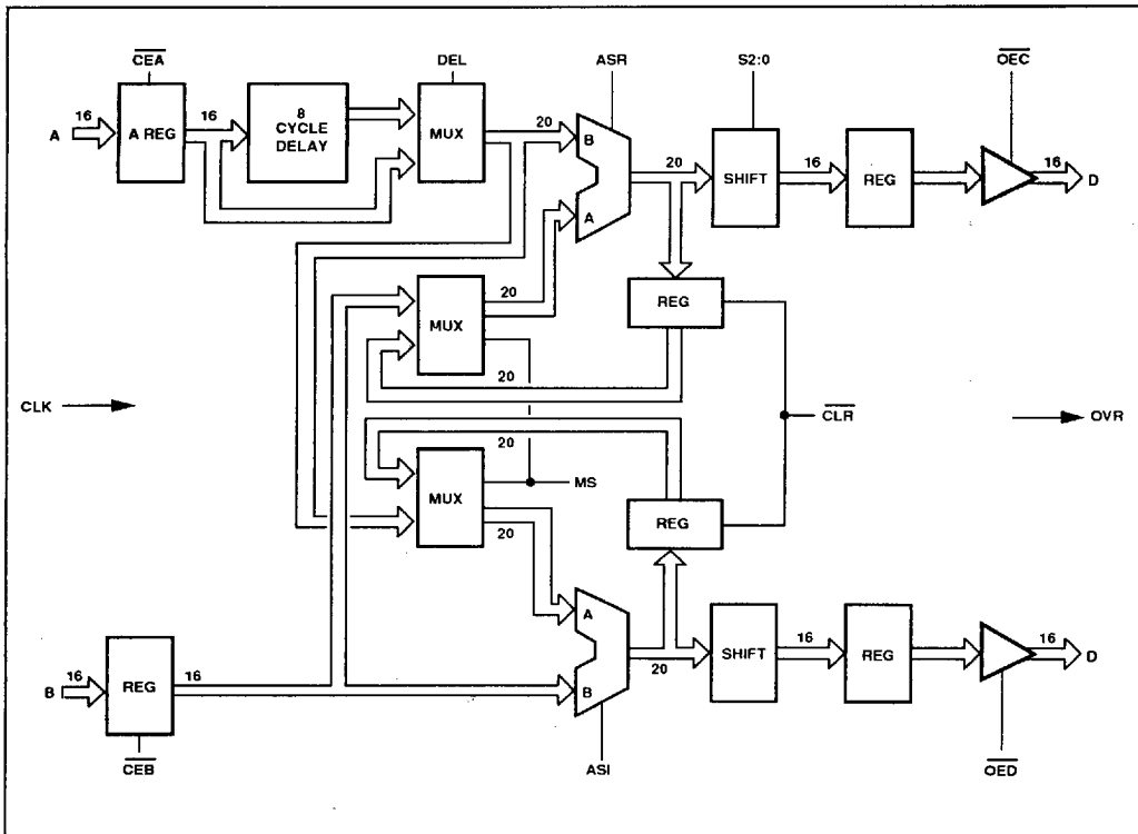
Fig. 3 Block diagram
