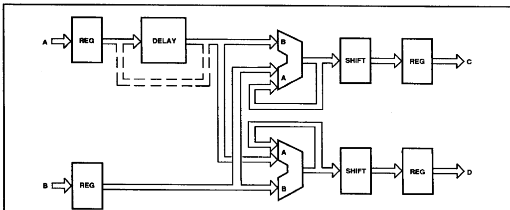
Fig. 2 PDSP16318 simplified block diagram
