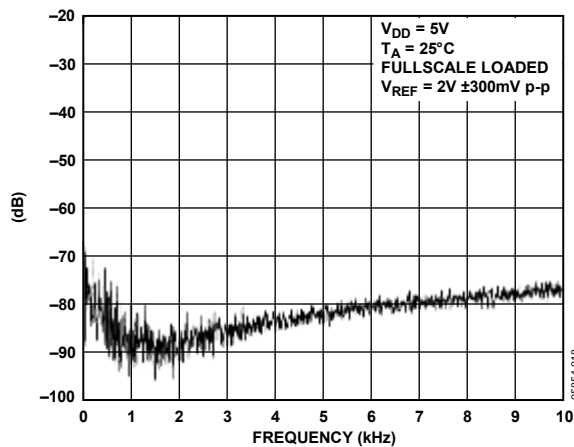
Figure 18. Total Harmonic Distortion
