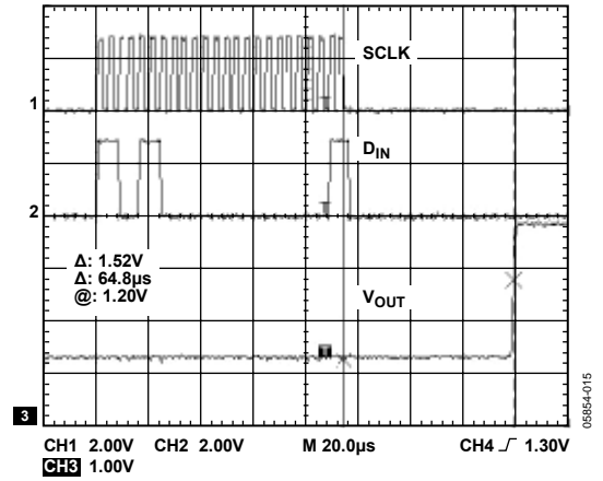
Figure 13. Full-Scale Settling Time, 5V
