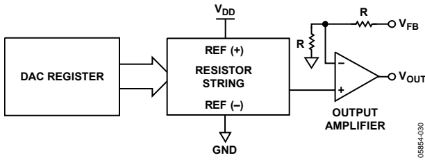
Figure 22. DAC Architecture
