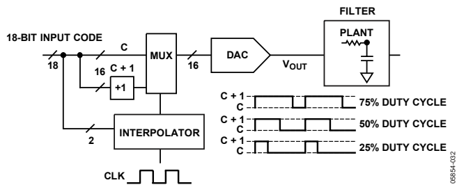
Figure 24. Interpolation Architecture
