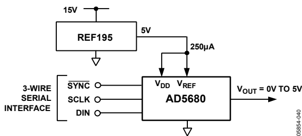
Figure 35. REF195 as Power Supply to the AD5680
