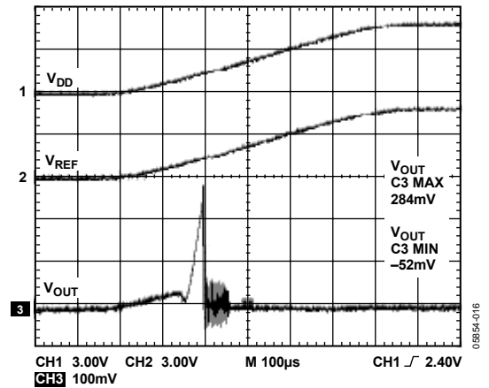
Figure 14. Power-On Reset to 0V
