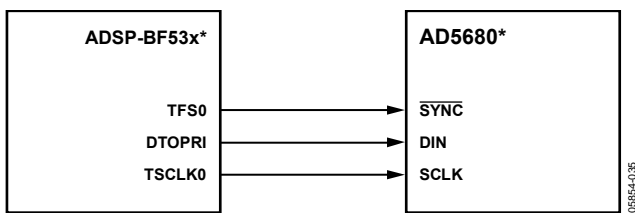
Figure 27. AD5680 to Blackfin ADSP-BF53x Interface
