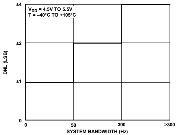
Figure 6. DNL Performance vs. System Bandwidth
