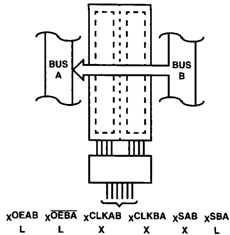
FIGURE 1. REAL-TIME TRANSFER BUS B TO A
