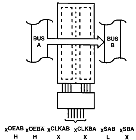
FIGURE 2. REAL-TIME TRANSFER BUS A TO B
