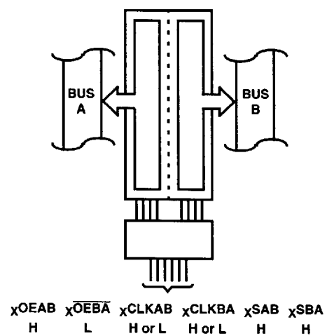
FIGURE 4. TRANSFER STORES DATA TO A AND/OR B
