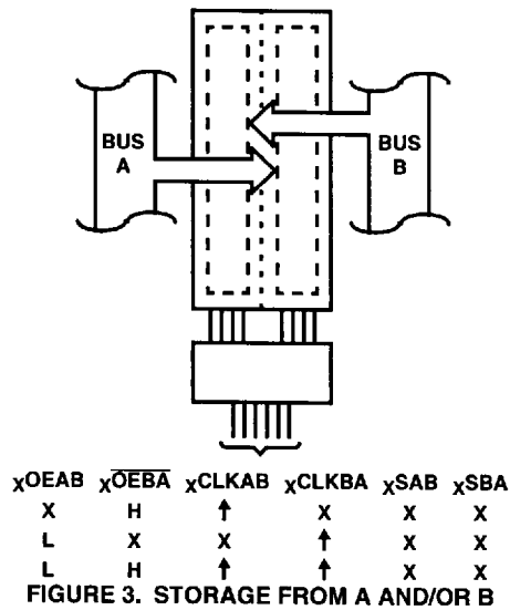
FIGURE 3. STORAGE FROM A AND/OR B
