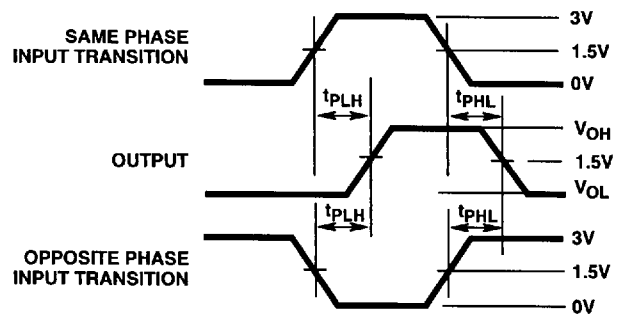
FIGURE 9. PROPAGATION DELAY
