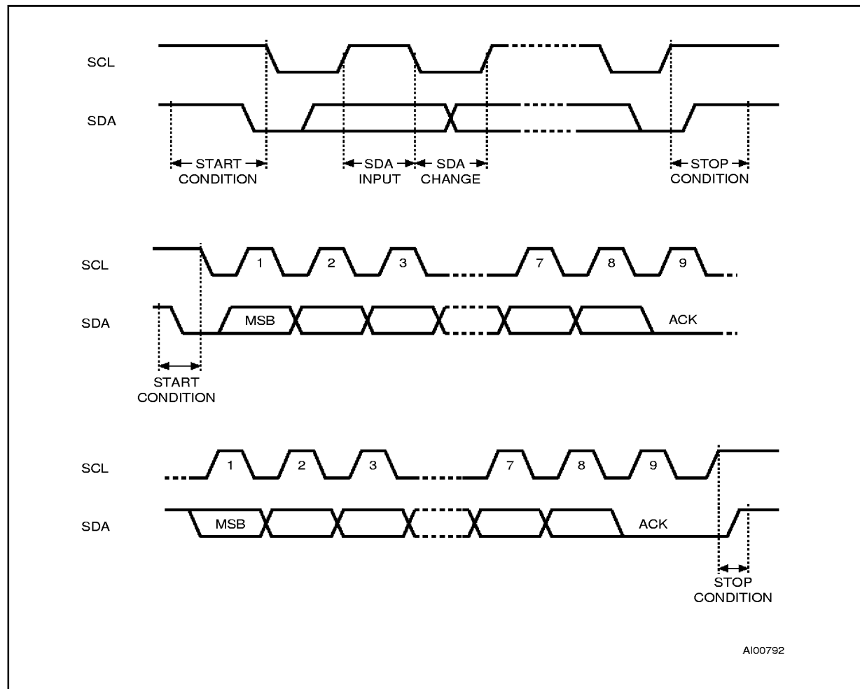
Figure 6. I 2 C Bus Protocol
