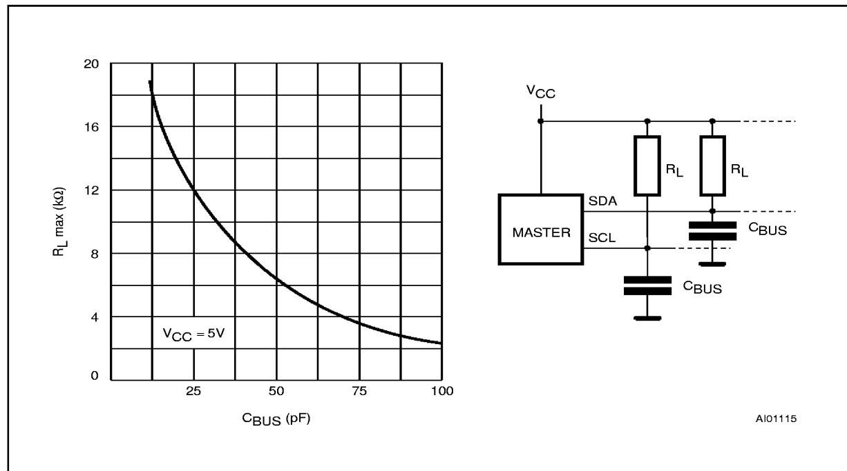
Figure 3. Maximum R_L Value versus Bus Capacitance ( C_{BUS} ) for an I 2 C Bus, f_C = 400\text{kHz}
