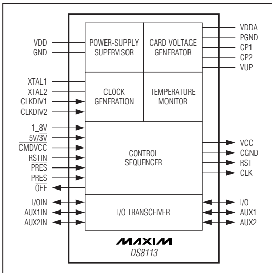
Figure 1. Functional Diagram
