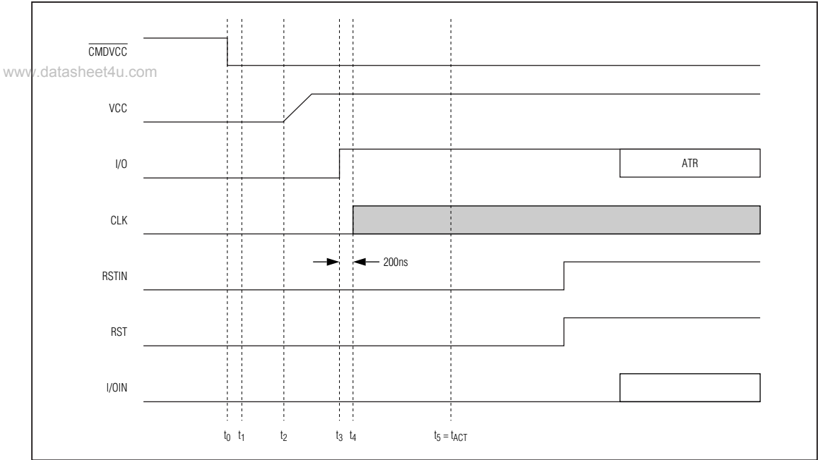
Figure 4. Activation Sequence at t_3
