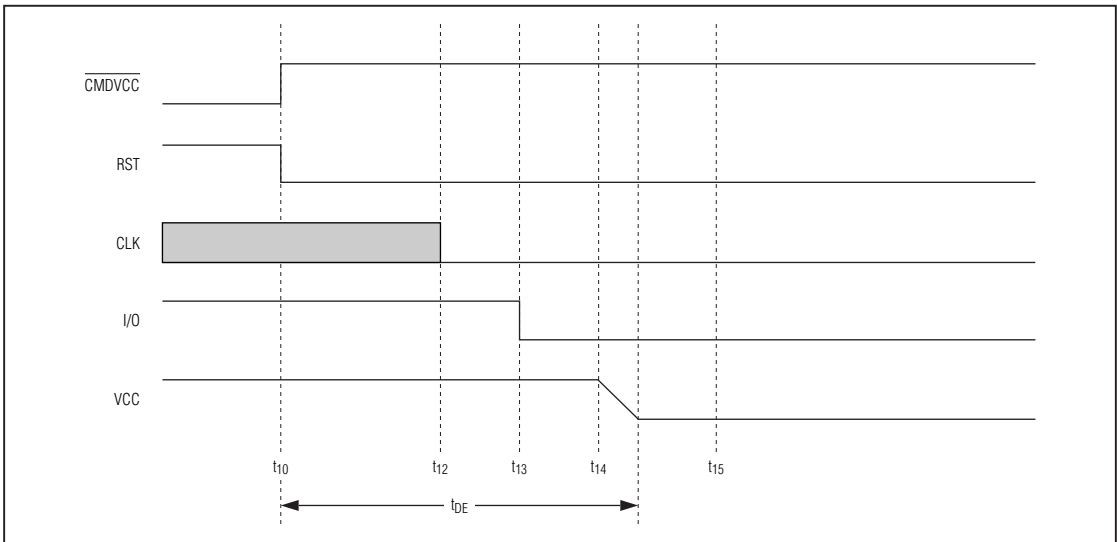
Figure 5. Deactivation Sequence
