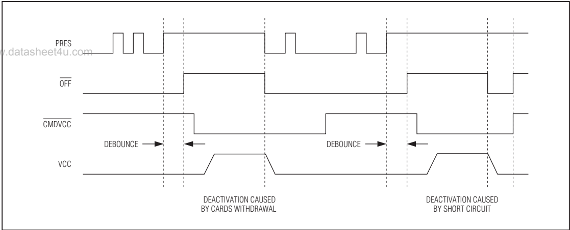
Figure 6. Behavior of PRES, \overline{\text{OFF}} , \overline{\text{CMDVCC}} , and VCC
