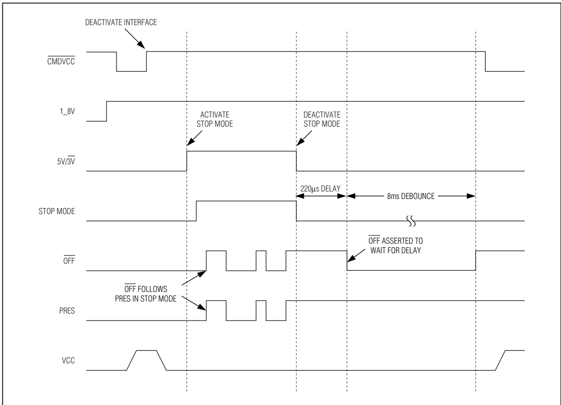
Figure 8. Stop-Mode Sequence
