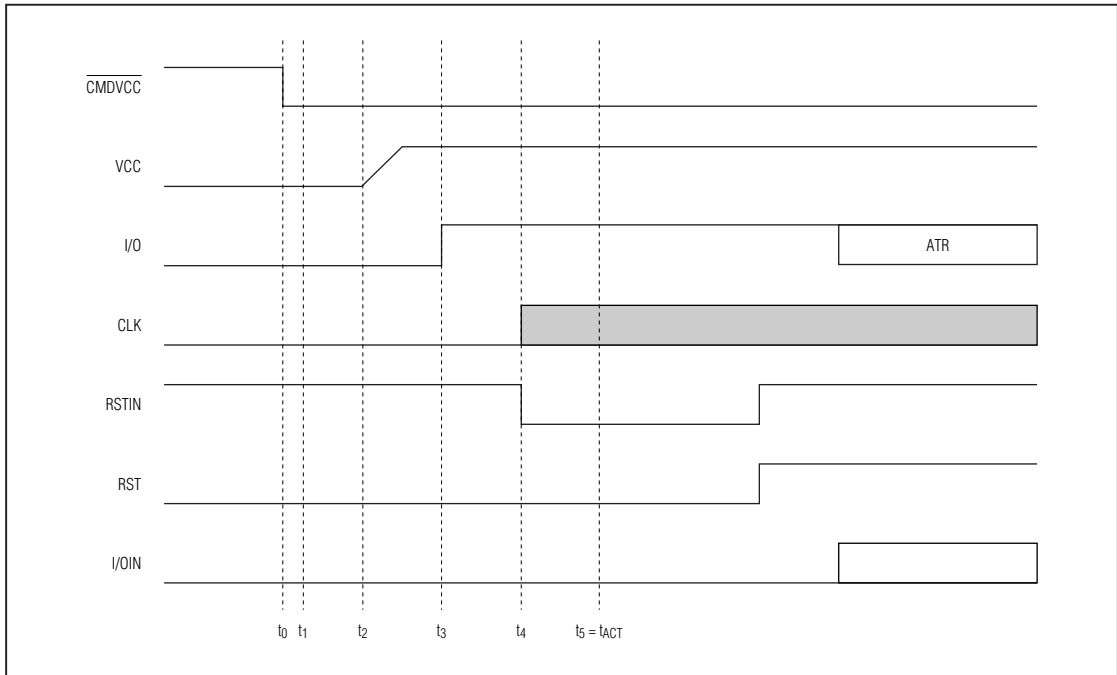
Figure 3. Activation Sequence Using RSTIN and \overline{\text{CMDVCC}}
