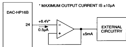
Figure 2. Use of Reference Output
