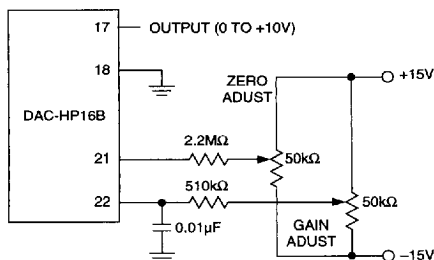
Figure 3. Unipolar Operations
