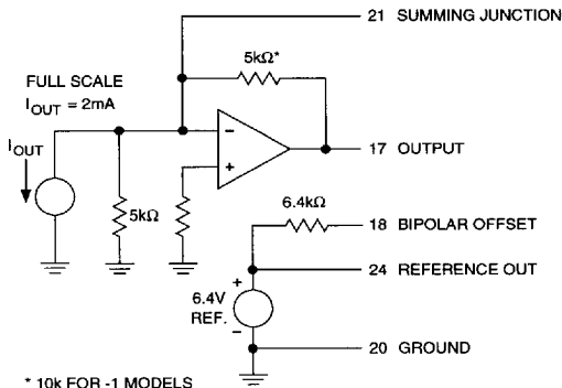
Figure 5. Output Circuit
