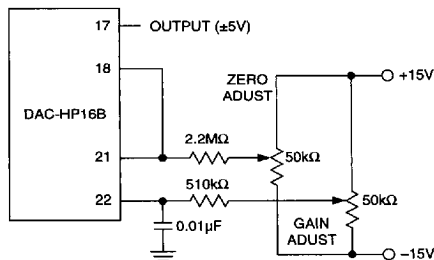
Figure 4. Bipolar Operations
