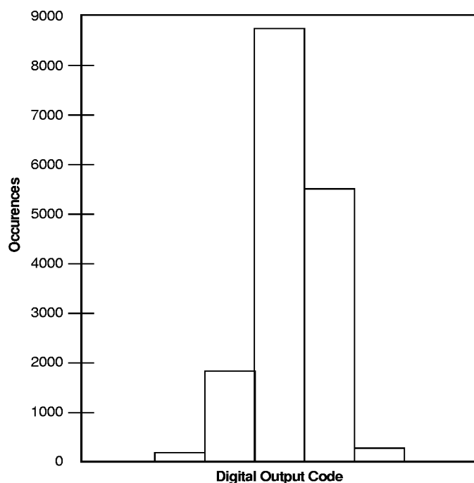
Figure 8. ADS-944 Grounded Input Histogram
