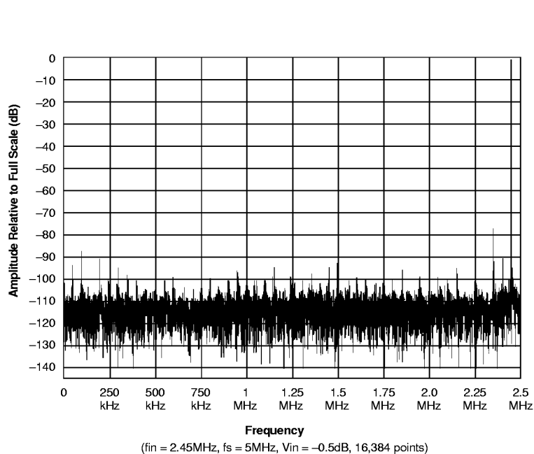
Figure 5. ADS-944 FFT
