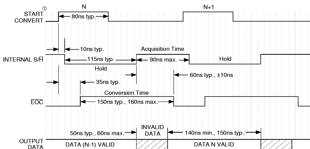
Figure 3. ADS-944 Timing Diagram
