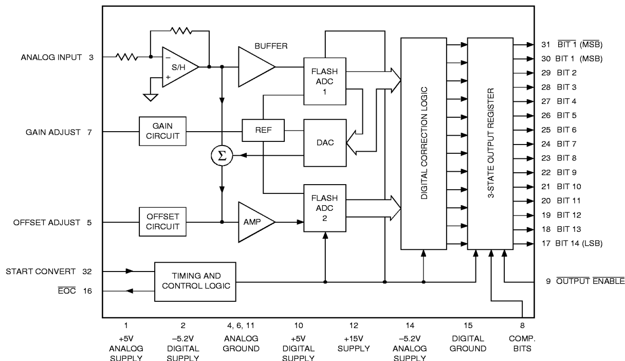
Figure 1. ADS-944 Functional Block Diagram
