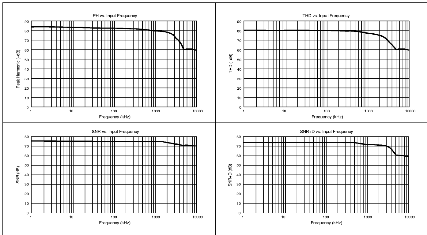
Figure 4. Typical ADS-944 Dynamic Performance vs. Input Frequency at +25°C
