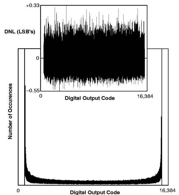
Figure 6. ADS-944 Histogram and Differential Nonlinearity
