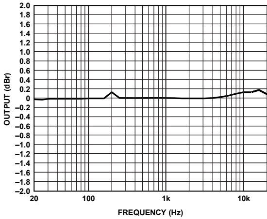
Figure 23. Frequency Response @ 1 W, 6 Ω, PVDD = 12 V, PGA = 0 dB
