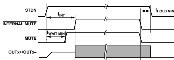
Figure 2. Timing Diagram (Minimum)
