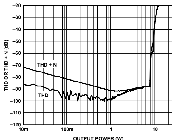
Figure 9. THD or THD + N vs. Output Power, 6 Ω, PVDD = 12 V
