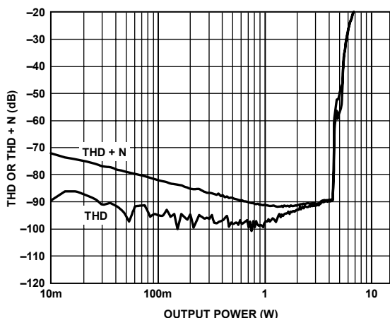
Figure 6. THD or THD + N vs. Output Power, 6 Ω, PVDD = 9 V
