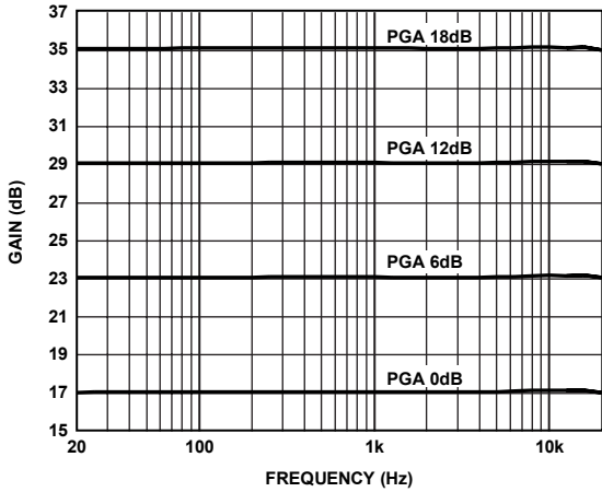
Figure 24. Gain vs. Frequency @ 1 W, 6 Ω, PVDD = 12 V, 6 Ω
