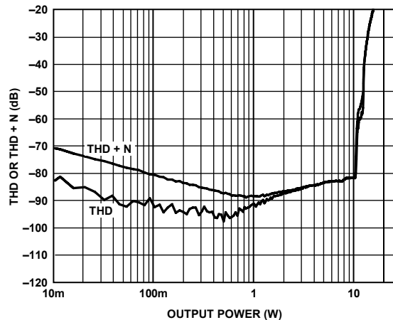
Figure 8. THD or THD + N vs. Output Power, 4 Ω, PVDD = 12 V
