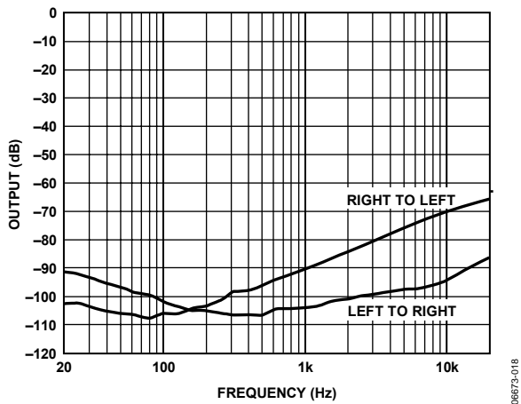
Figure 18. Crosstalk @ 1 W, 6 Ω, PVDD = 12 V, PGA = 0 dB
