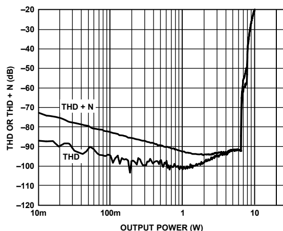
Figure 10. THD or THD + N vs. Output Power, 8 Ω, PVDD = 12 V
