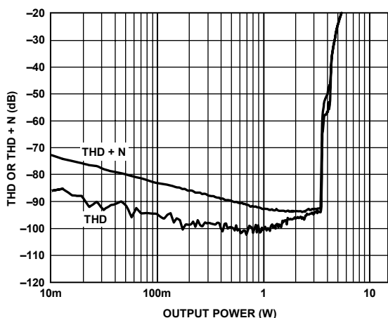
Figure 7. THD or THD + N vs. Output Power, 8 Ω, PVDD = 9 V
