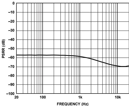
Figure 25. PSRR vs. Frequency, No Input Signal Ripple = 1.2 V p-p, PVDD = 12 V, 6 Ω
