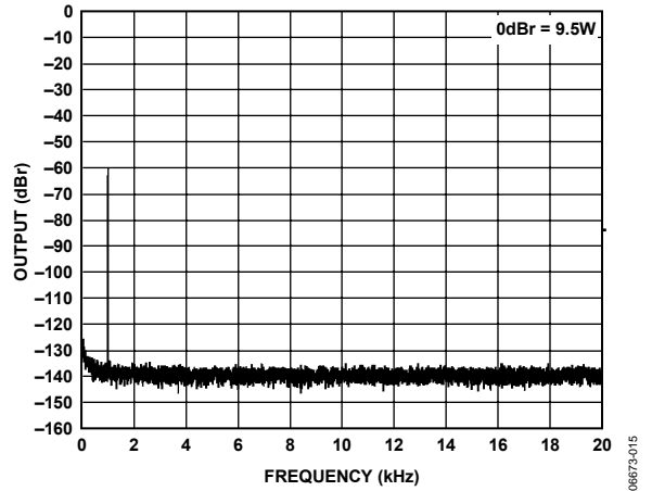
Figure 15. FFT @ -60 dBFS, 6Ω, PVDD = 12 V, PGA = 0 dB, 1 kHz Sine
