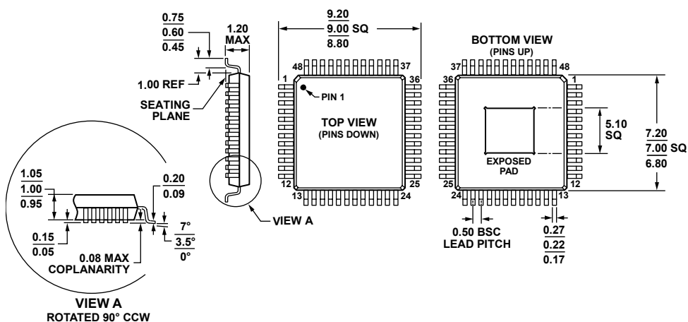
COMPLIANT TO JEDEC STANDARDS MS-026-ABC Figure 49. 48-Lead Thin Quad Flat Package, Exposed Pad [TQFP_EP] (SV-48-5) Dimensions shown in millimeters
