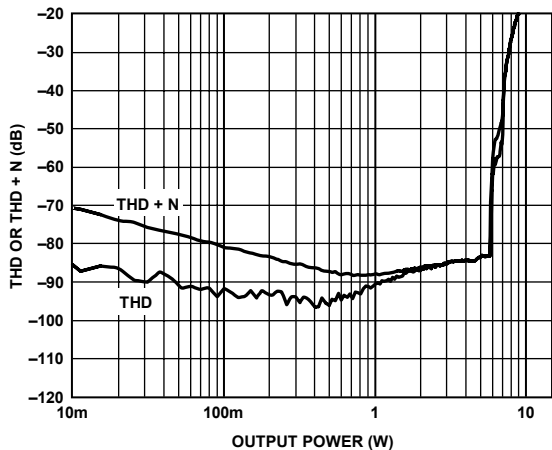
Figure 5. THD or THD + N vs. Output Power, 4 Ω, PVDD = 9 V
