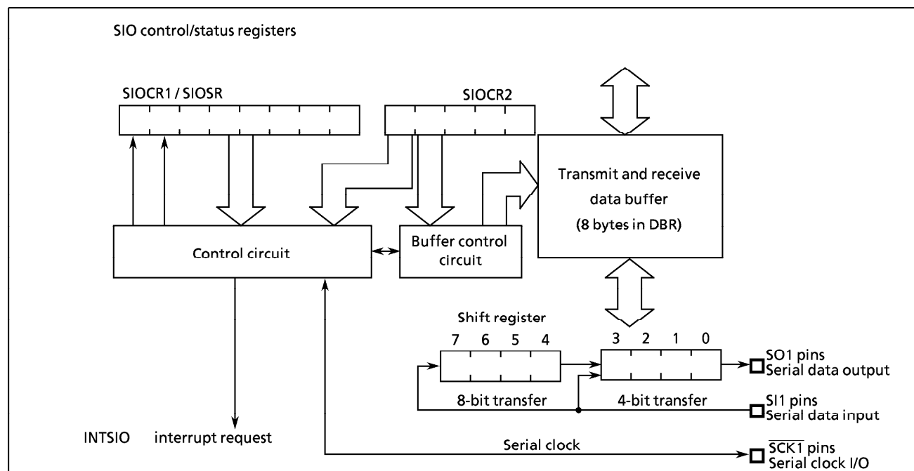
Figure 2-32. Serial Interfaces
