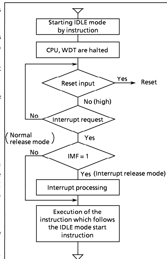
Figure 1-19. IDLE Mode
