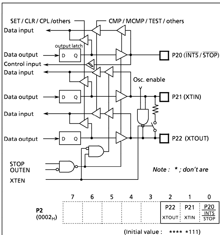
Figure 2-5. Port P2
