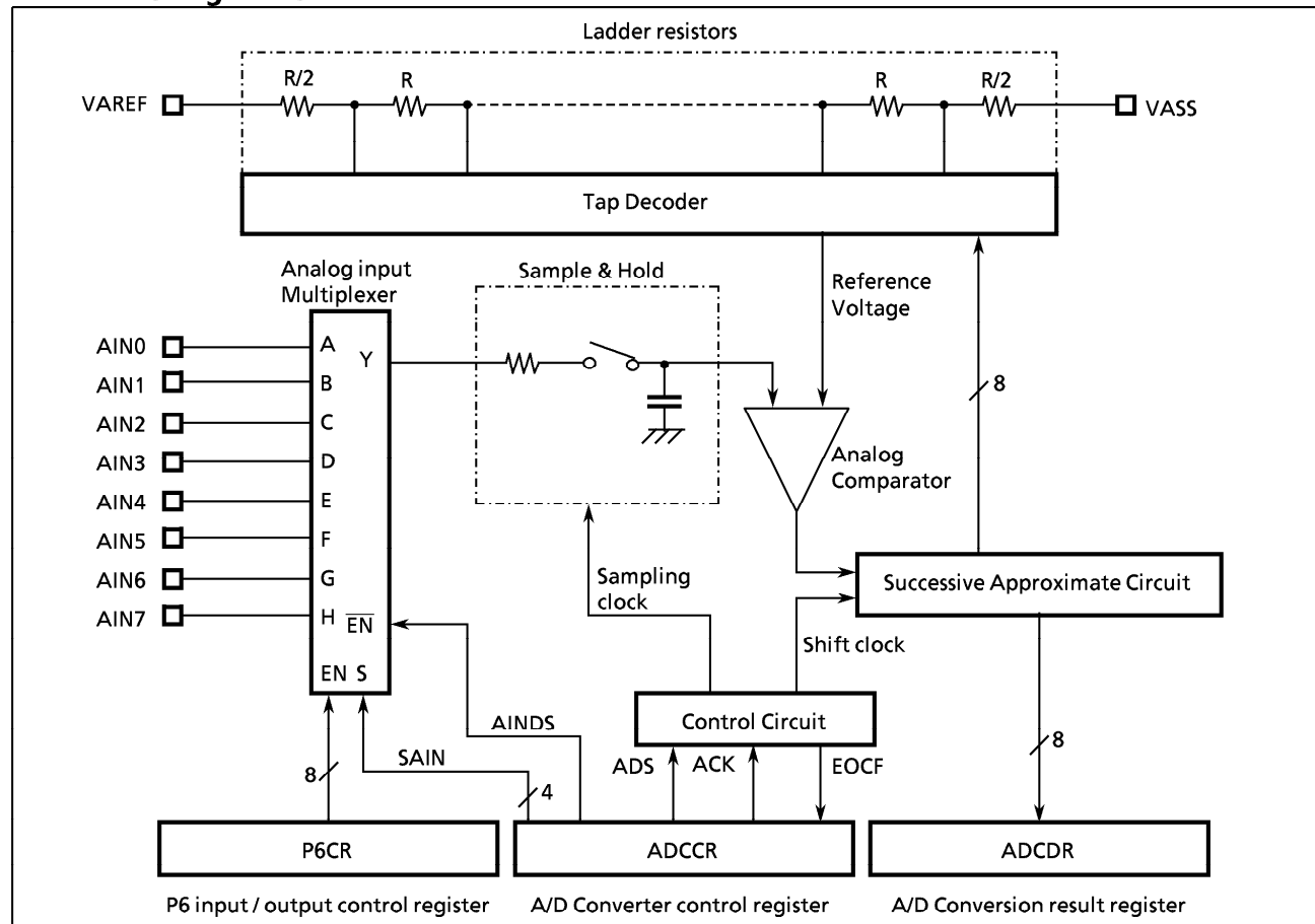
Figure 2-44. A/D Converter
