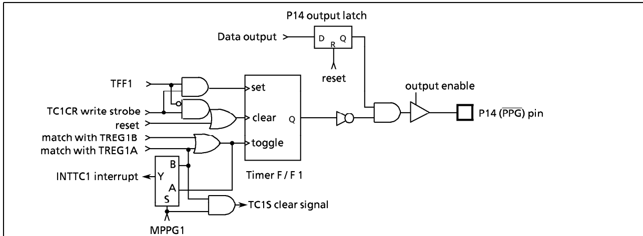
Figure 2-21. PPG Output
