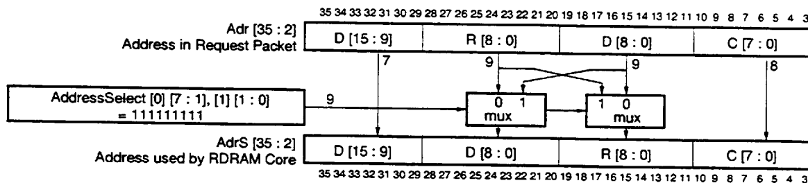
Figure 9-1. AddressMapping Hardware
