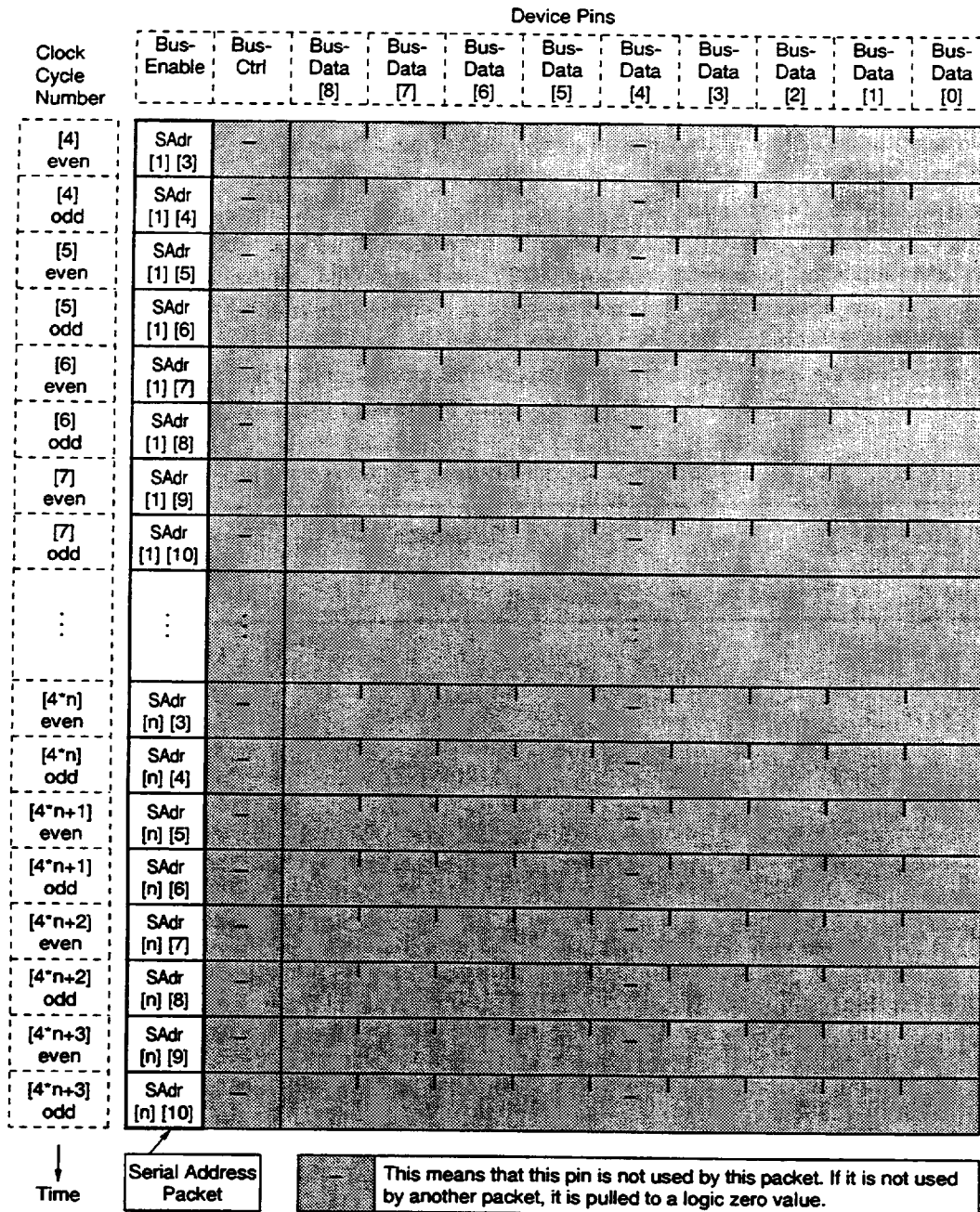
Figure 5-5. Serial Address Packet Format
