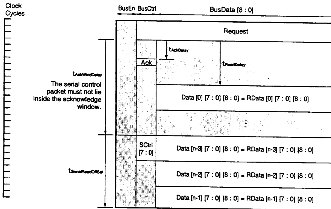
Figure 7-5. Read Transaction with Serial Control Packet
