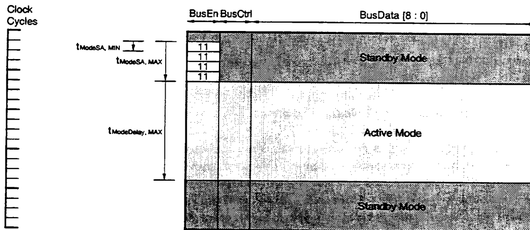
Figure 6-2. Basic ActiveMode/StandbyMode Transitions
