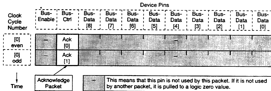
Figure 5-2. Acknowledge Packet Format
