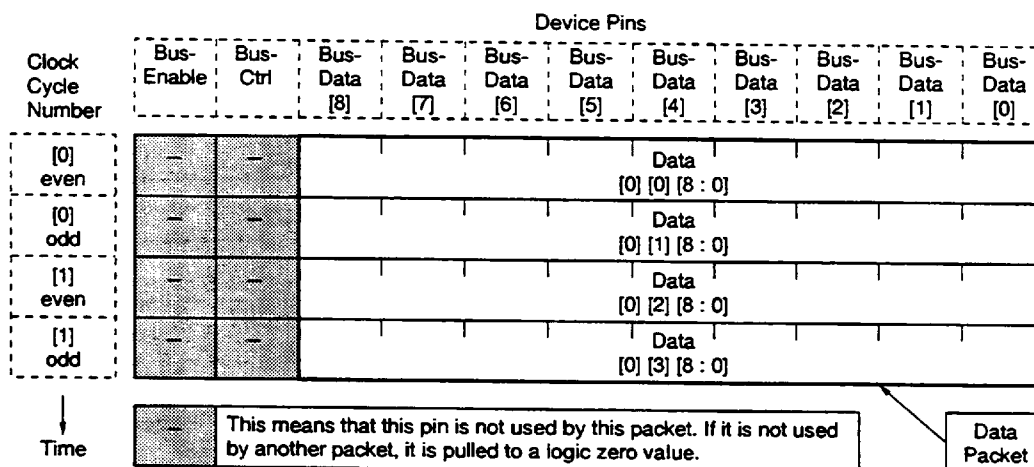
Figure 5-3. Data Packet Format (Register Space)
