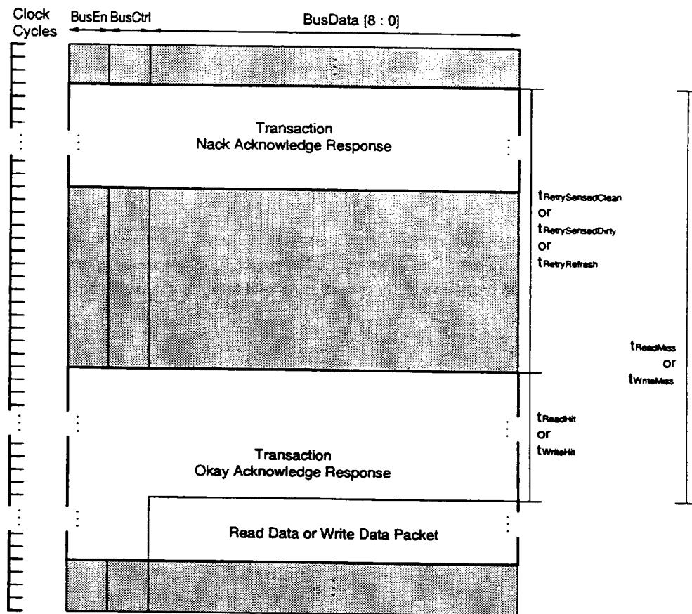
Figure 8-1. Nack Acknowledge Response
