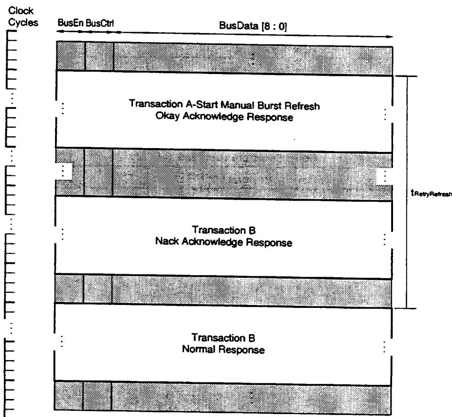
Figure 8-2. Transaction Holdoff Due to Burst Refresh
