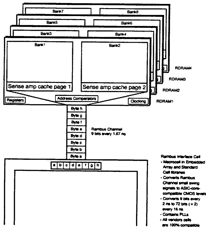
Figure 3-1. Converting the Channel Data Rate
