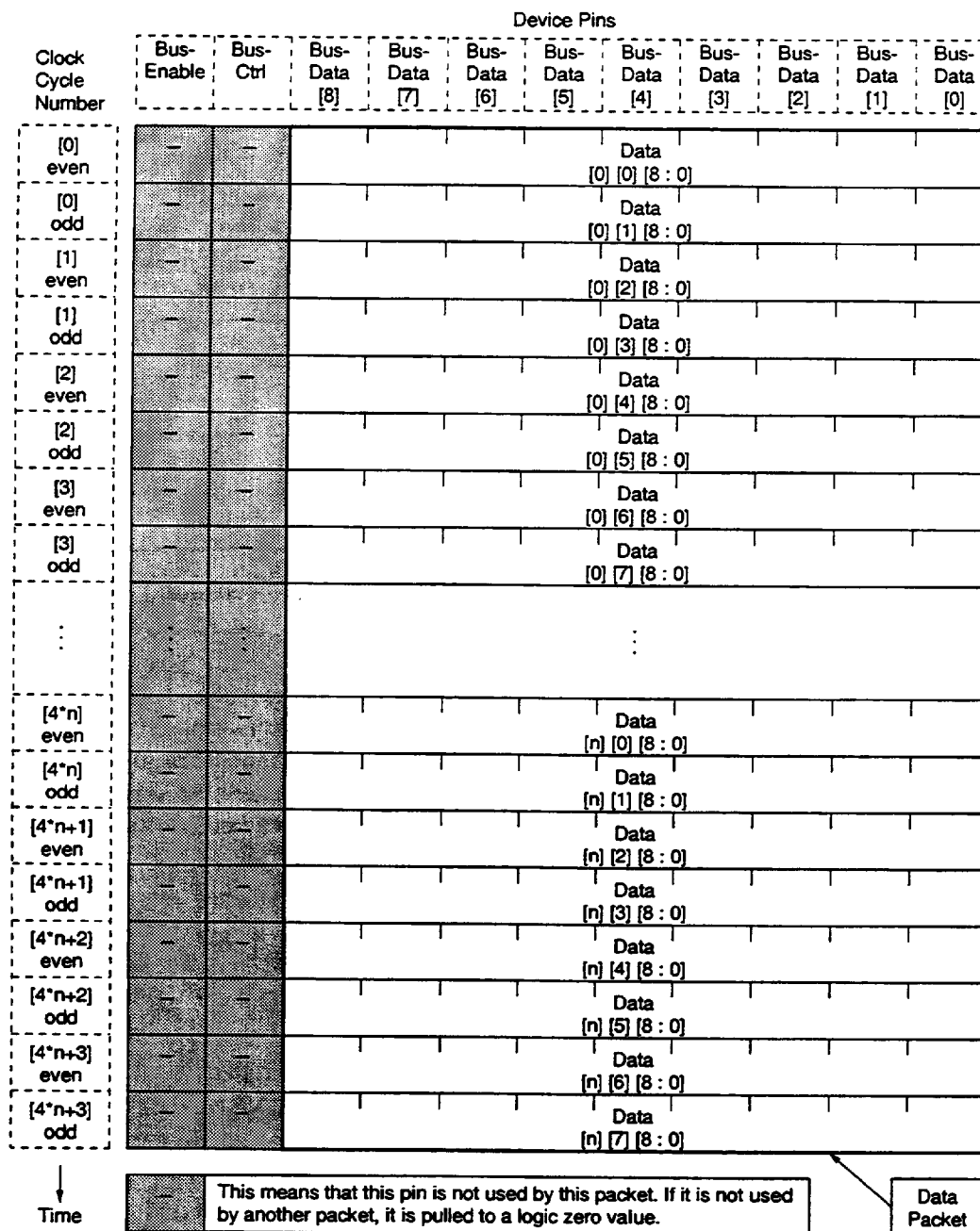
Figure 5-4. Data Packet Format (Memory Space)
