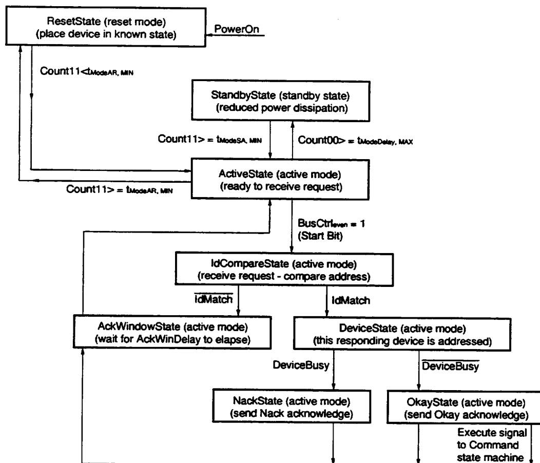
Figure 6-1. Frame State Machine - State Diagram
