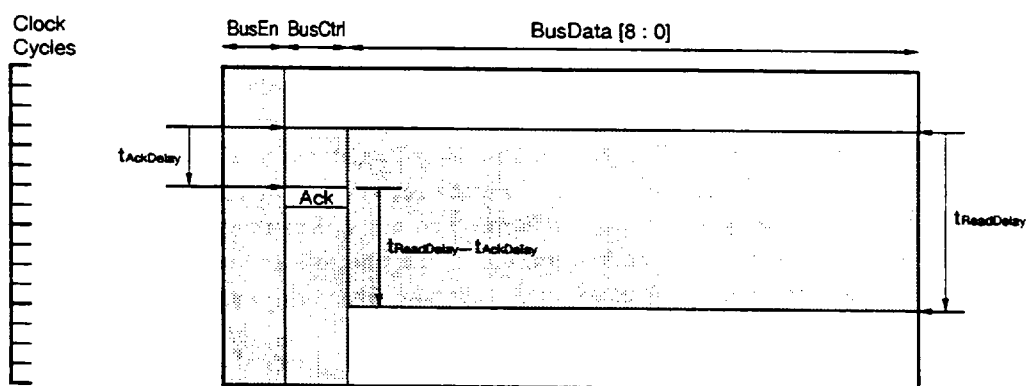
Figure 7-1. Read Transaction
