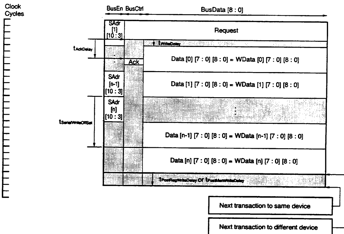
Figure 7-4. Write Transaction with Serial Address Packet
