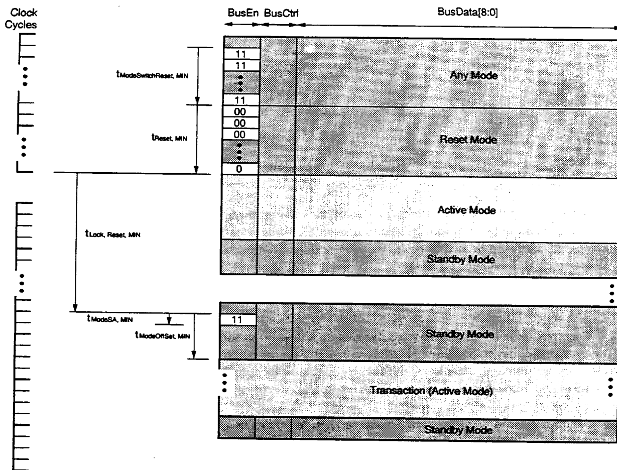
Figure 6-4. ResetMode to ActiveMode Transition
