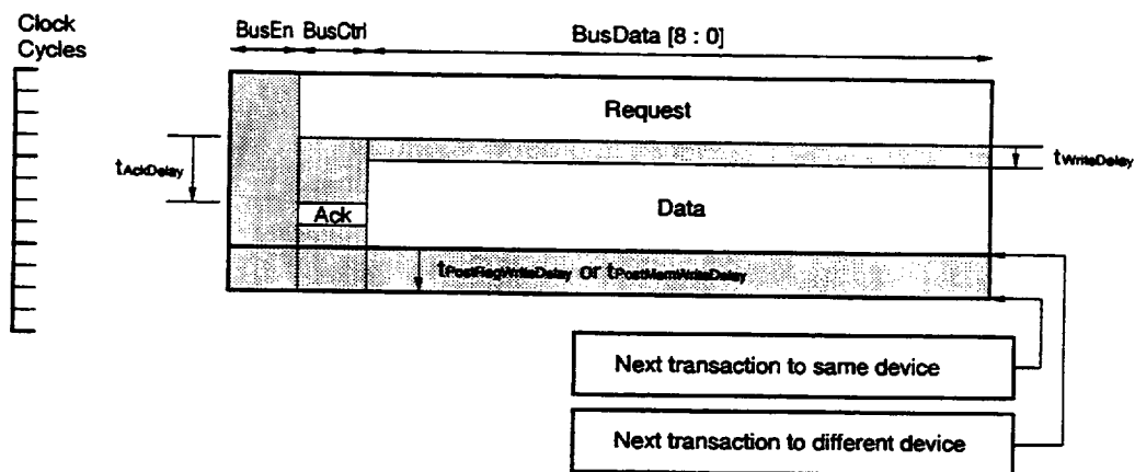
Figure 7-2. Write Transaction
