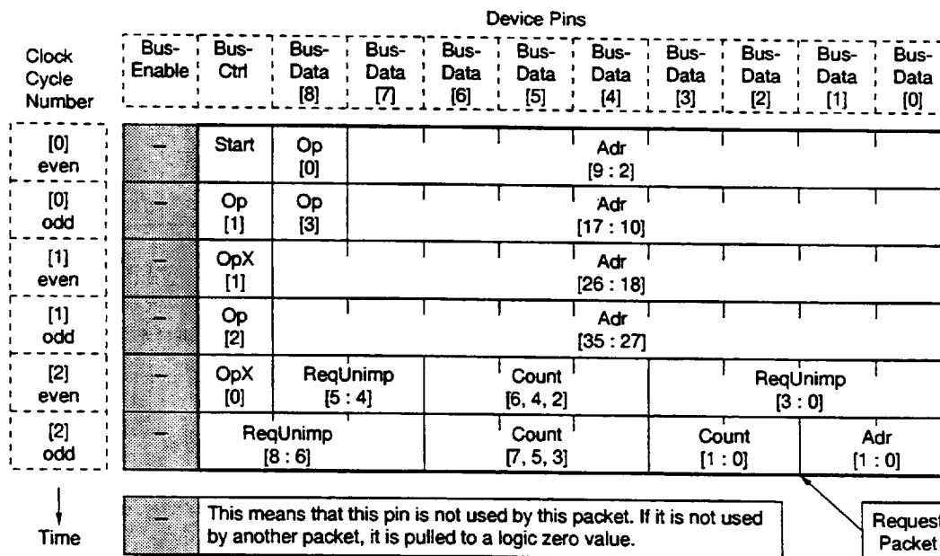
Figure 5-1. Request Packet Format
