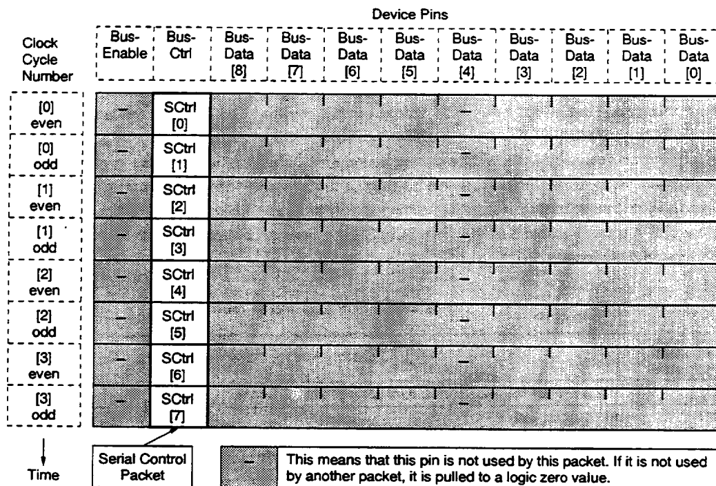
Figure 5-6. Serial Control Packet Format
