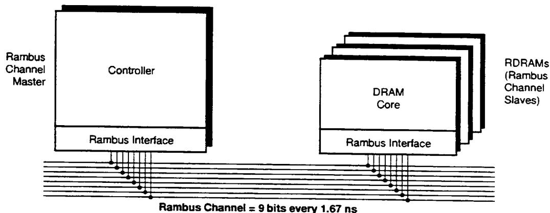
Figure 2-1. Logical Representation
