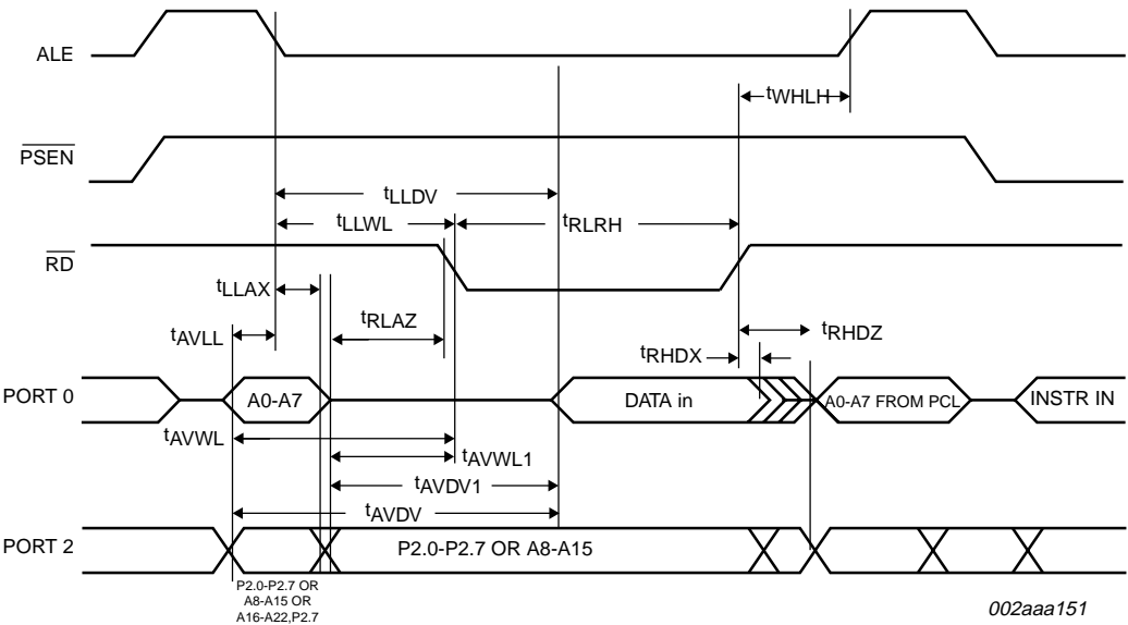
Fig 5. External data memory read cycle (non-extended memory cycle).
