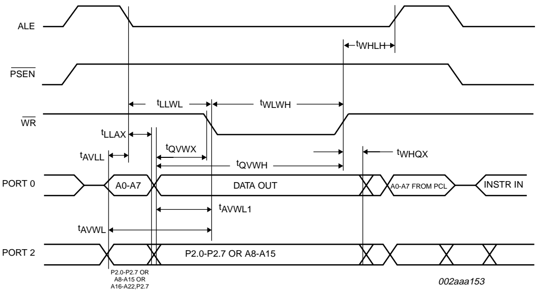
Fig 6. External data memory write cycle (non-extended memory cycle).
