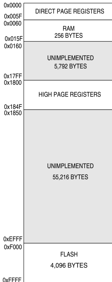
Figure 4-1. MC9S08QD4 Memory Map
