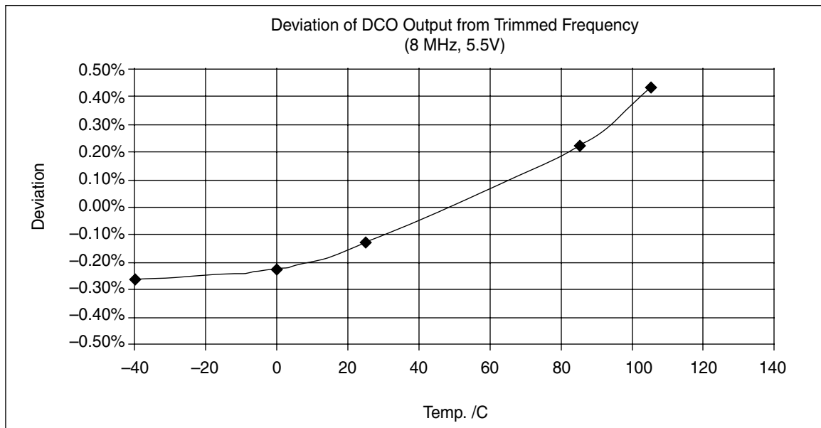
Figure A-10. Typical Deviation of DCO Output vs Temperature
