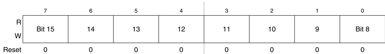
Figure 11-9. Timer Channel Value Register High (TPMxCnVH)
