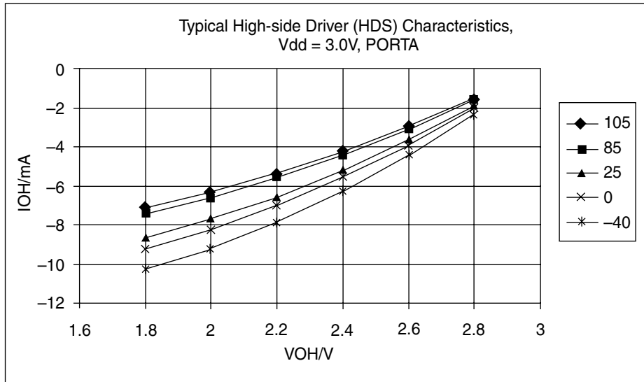
Figure A-8. Typical High-Side Driver (Source) Characteristics High Drive (PTxDSn = 1), V dd = 3.0V, VOH vs IOH
