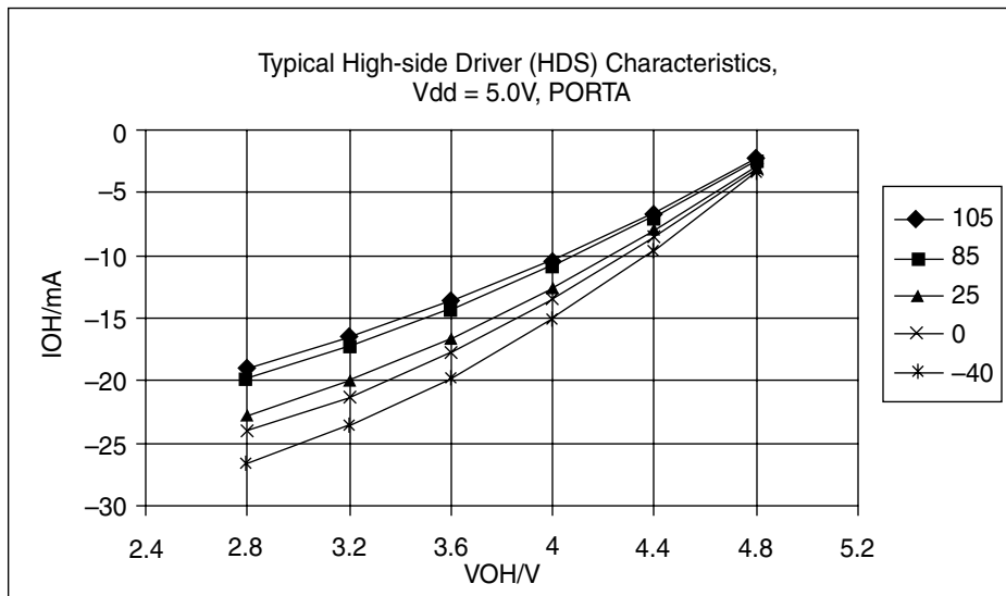
Figure A-7. Typical High-Side Driver (Source) Characteristics High Drive (PTxDSn = 1), Vdd = 5.0V, VOH vs IOH
