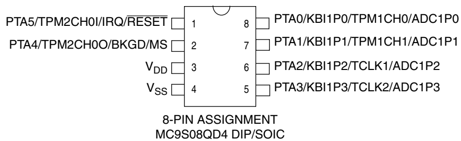
Figure 2-1. 8-Pin Packages
