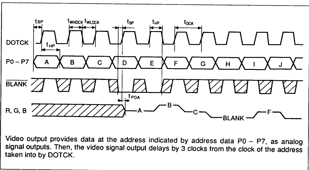
Figure 9 Video Output
