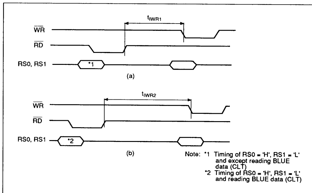
Figure 6 Write after Read Interval Timing
