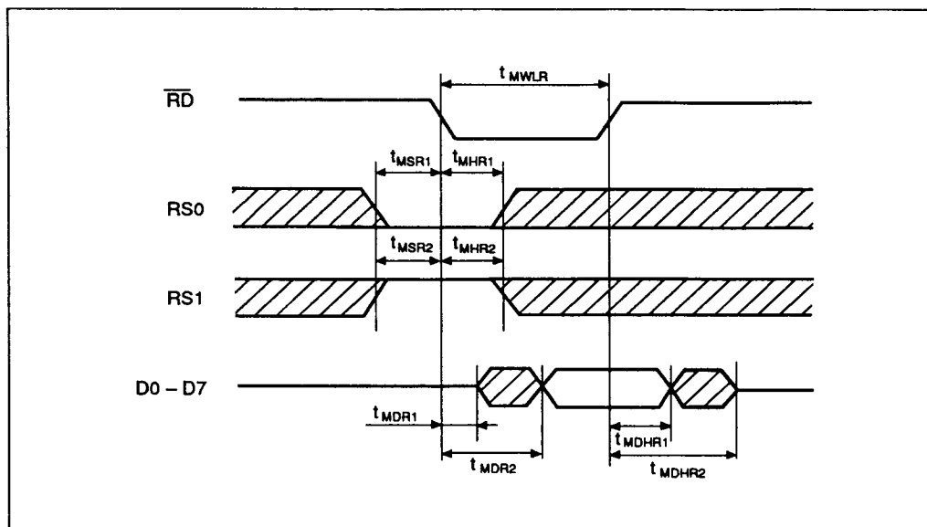
Figure 14 Read Out from Pixel Mask Register
