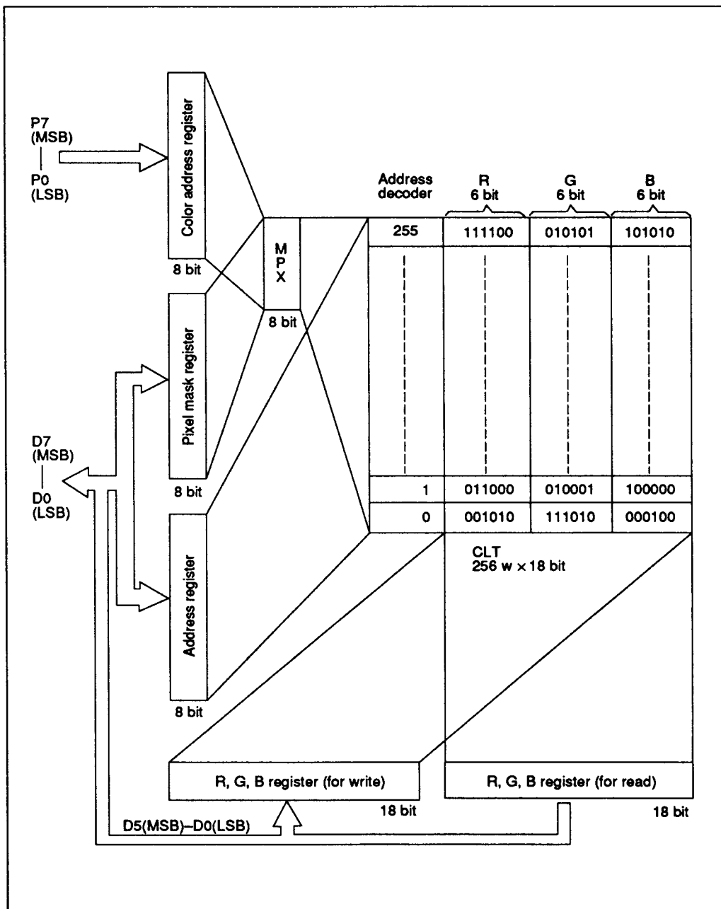
Figure 19 Correspondence of CLT with Each Register
