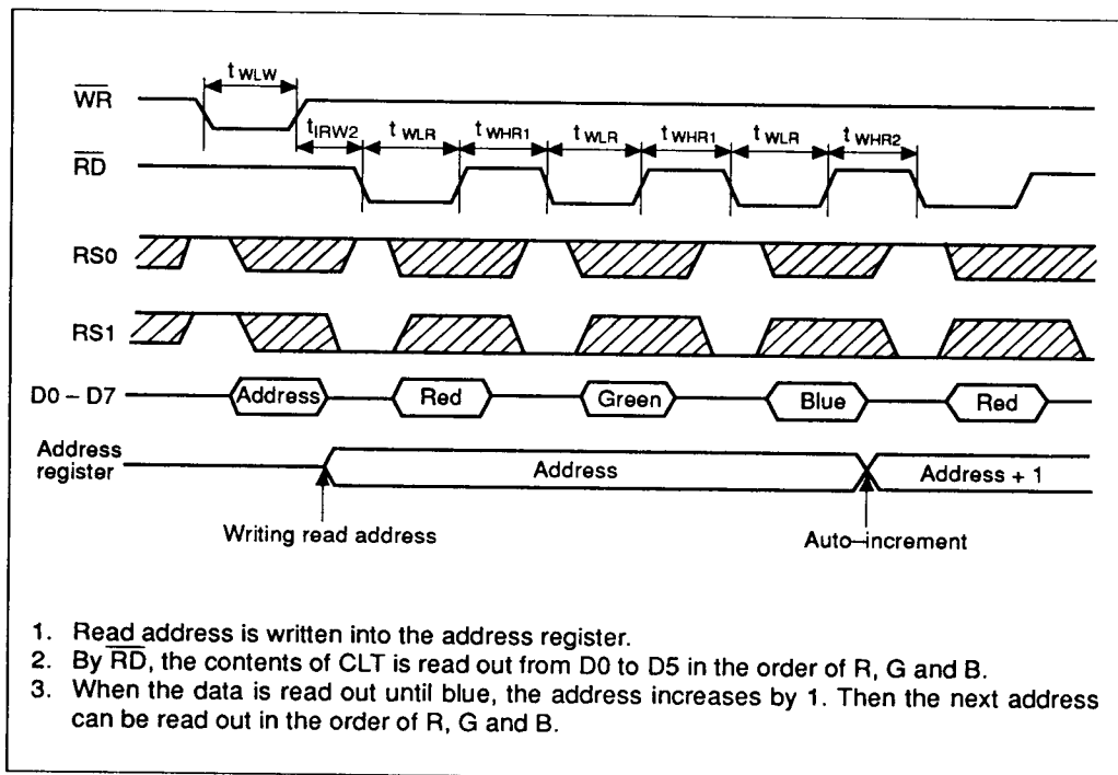
Figure 8 Read Out from CLT
