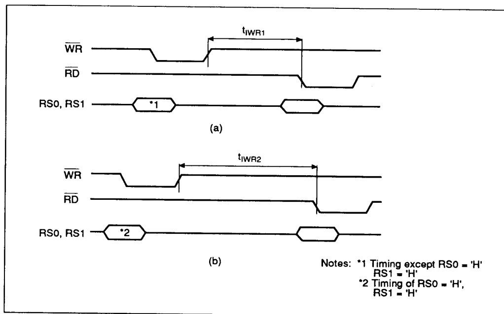
Figure 5 Read after Write Interval Timing
