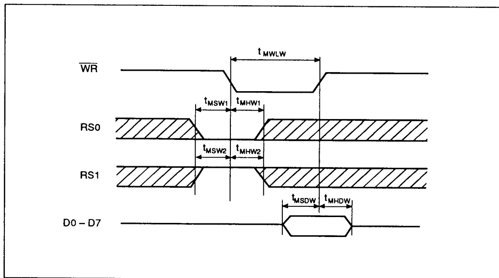
Figure 13 Data Write to Pixel Mask Register
