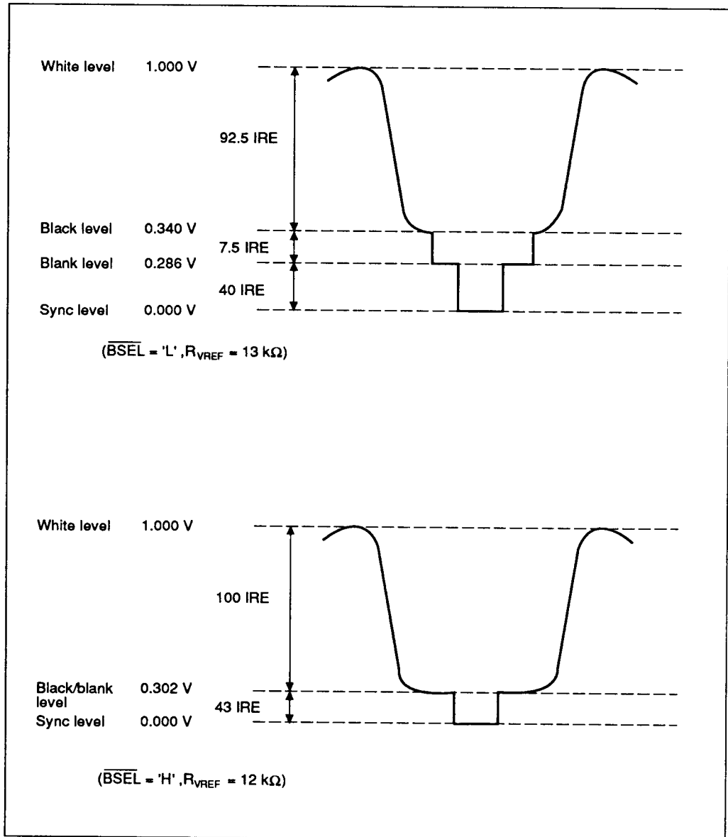
Figure 15 HD153109CP and HD153109MA VIDEO Output Waveform (In case of SYNC signal composite)
