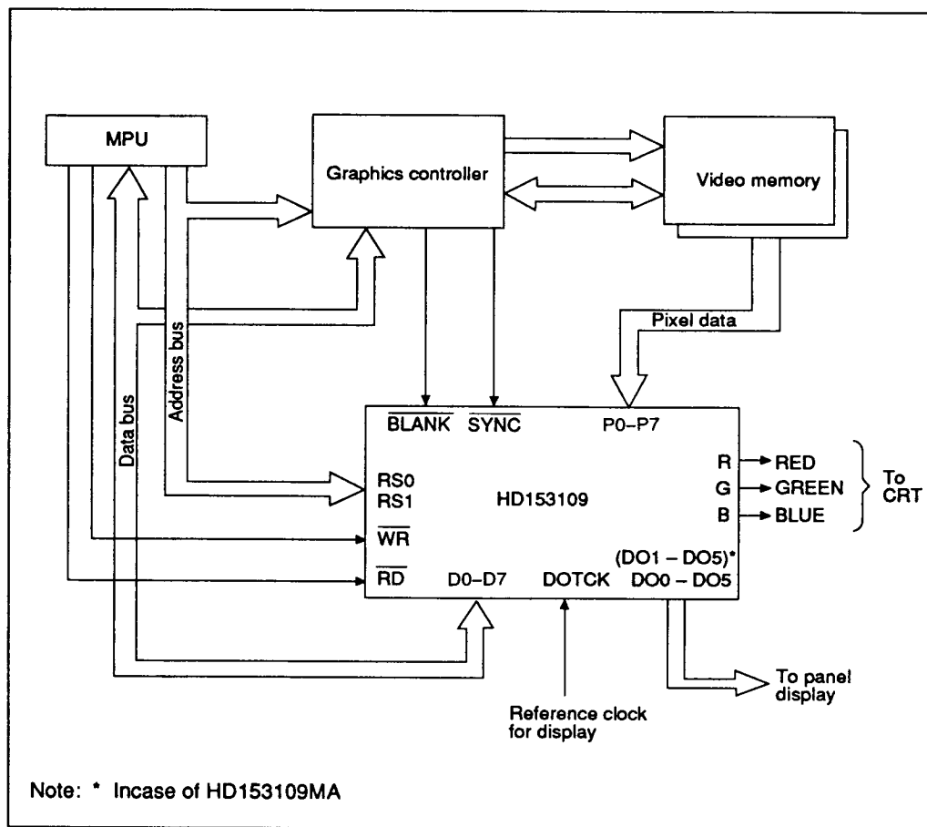
Figure 20 Example Construction of a Standard System
