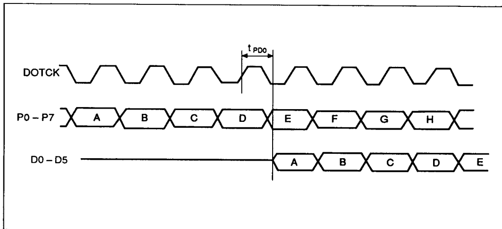
Figure 12 Digital Output
