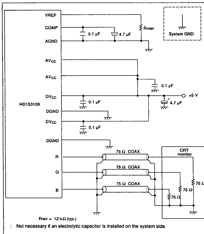
Figure 21 Example of External Parts
