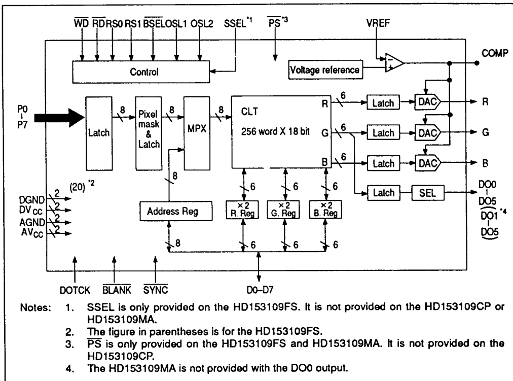
Figure 2 Block Diagrams
