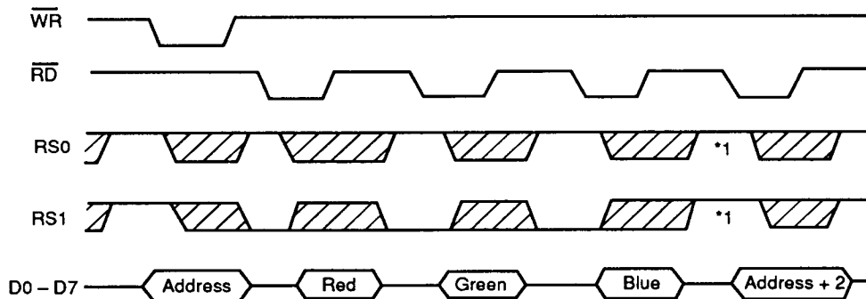
Figure 10 Read Out of Address Register (1)
