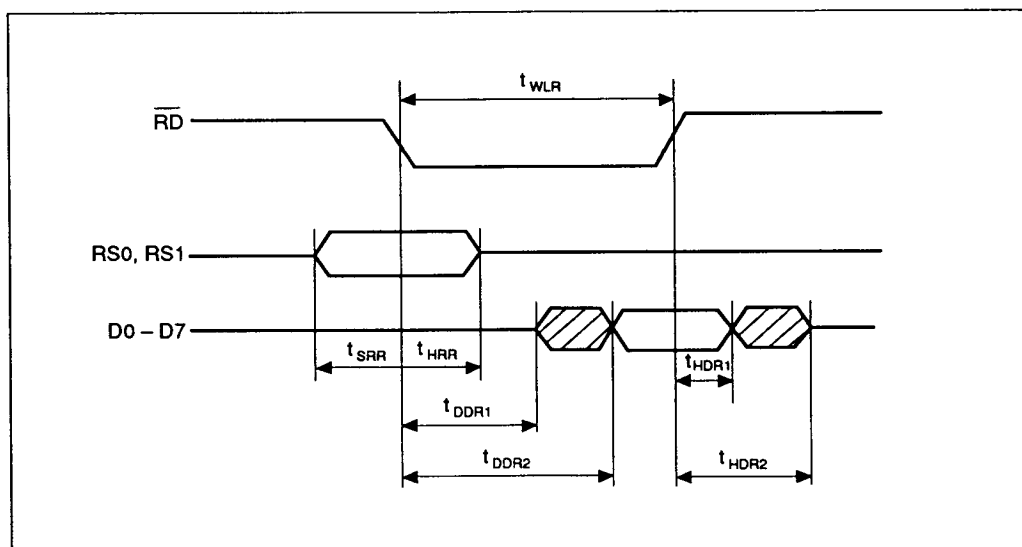
Figure 4 Data Read Out Timing
