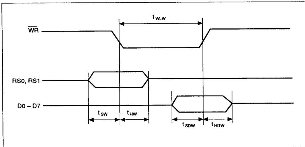
Figure 3 Data Write Timing
