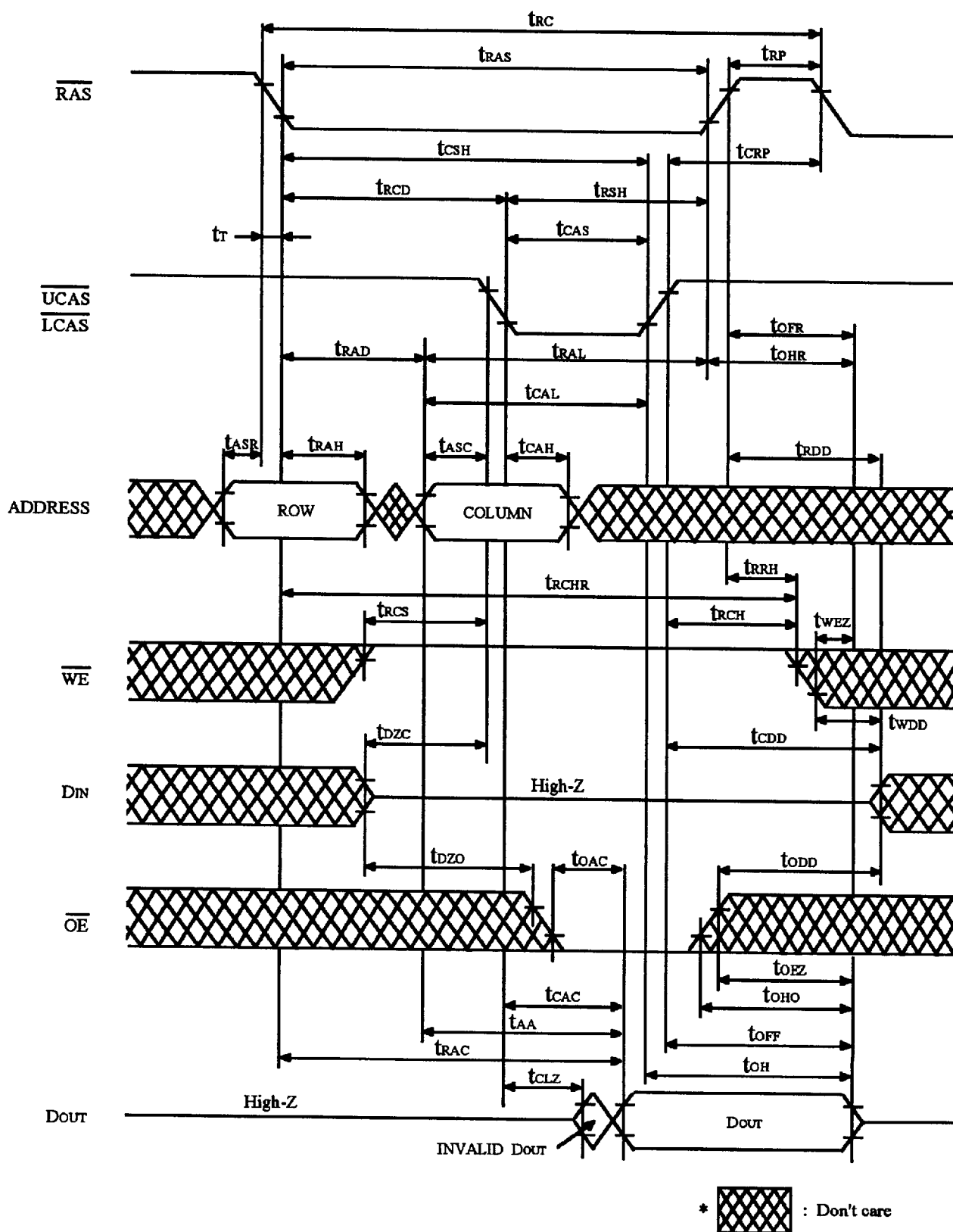
FIGURE 1. READ CYCLE
