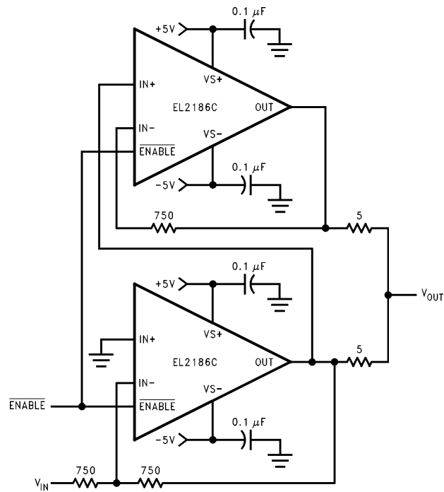
Inverting 200 mA Output Current Distribution Amplifier
