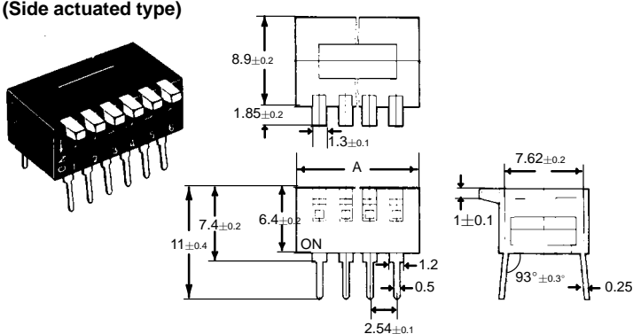
A6DR-□100 (Side actuated type)
