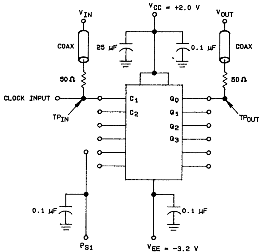
FIGURE 4. Test circuit and switching waveforms.
