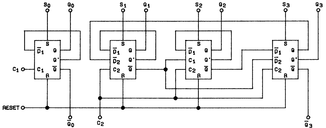
FIGURE 3. Logic diagram.
