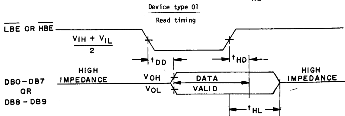
FIGURE 2. Timing diagrams.
