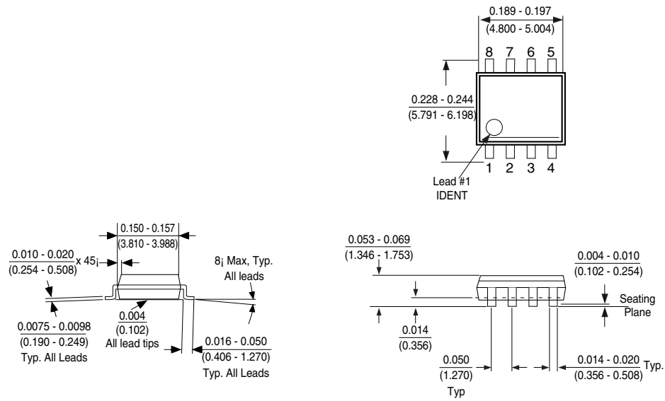
Molded Package, Small Outline, 0.15 Wide, 8-Lead (M8) Package Number M8A
