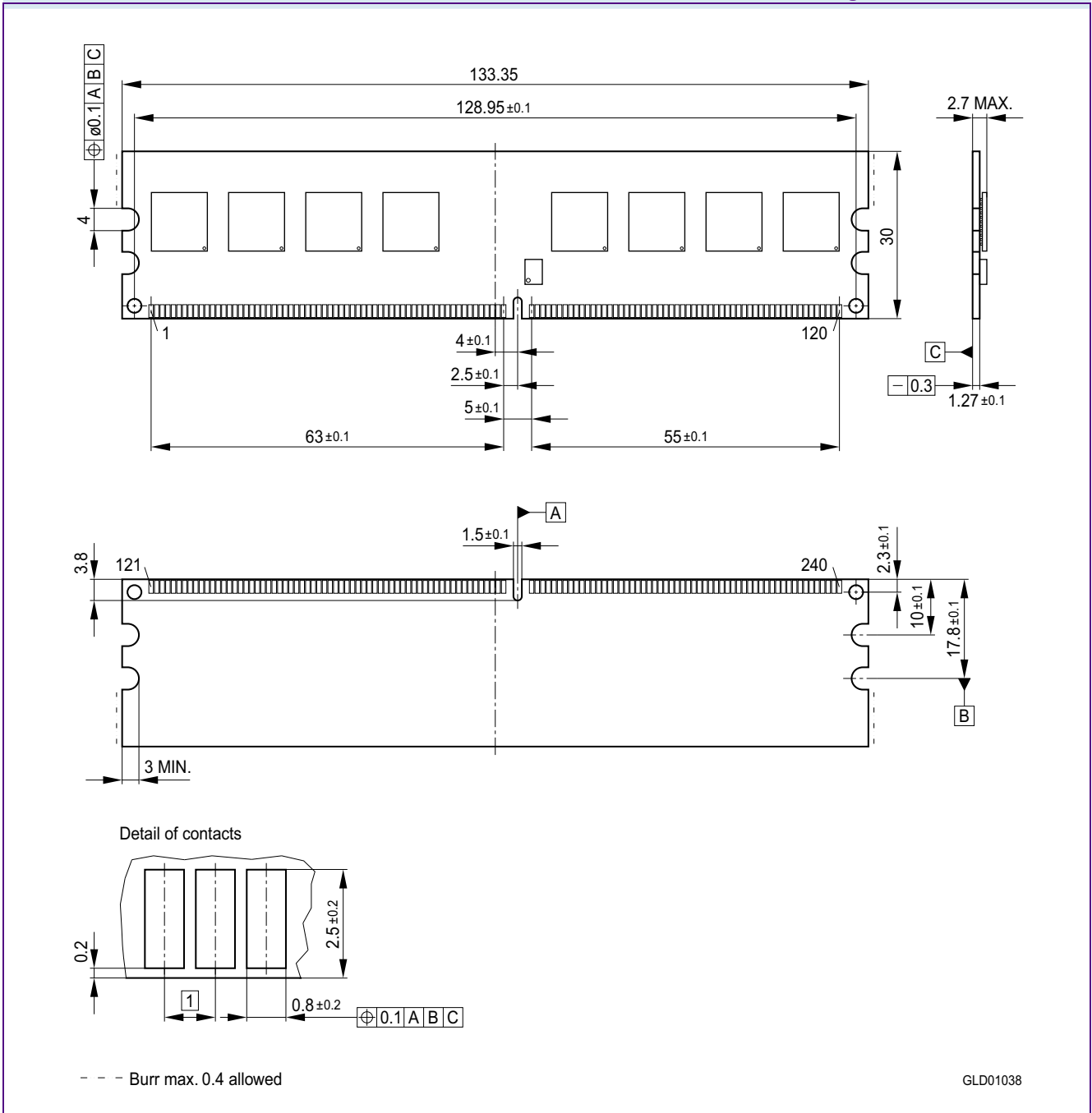
FIGURE 7 Package Outline L-DIM-240-8
