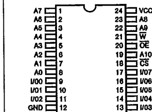
Pinout DIL 24 pins (top view)
