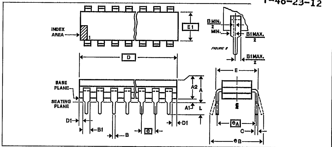
24 PINS CERDIP .600
