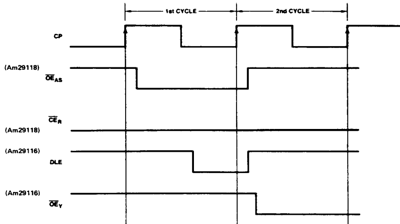
Figure 3. Timing Waveforms for Modifying R-Register in Two Microcycles using the Am29116.
