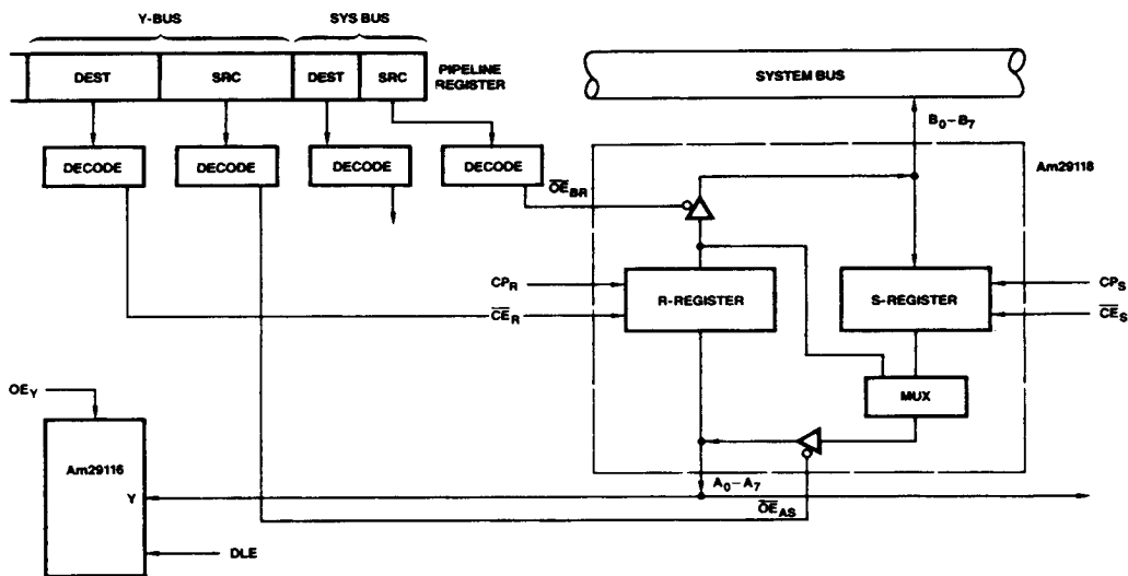
Figure 2. System Configuration.
