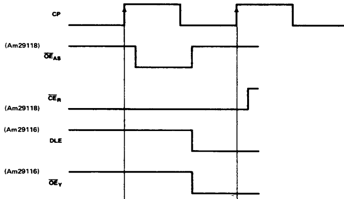
Figure 4. Timing Waveforms for Modifying R-Register using the Am29116.
